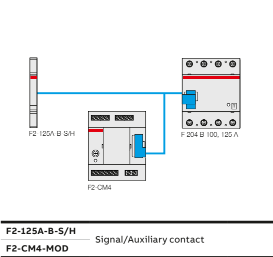
F200 B high ratings
