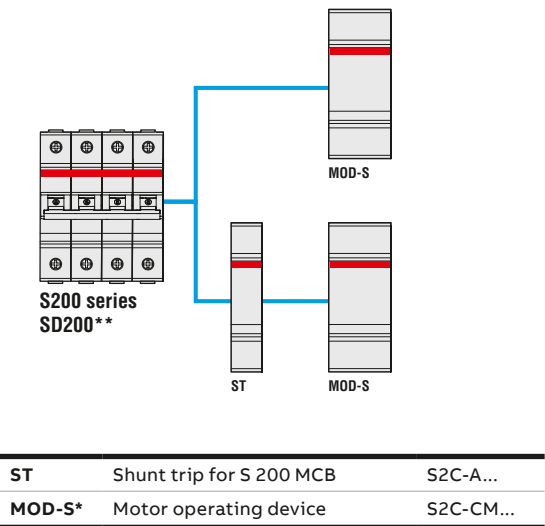
Combination of S200/SD200 with motor operating device
