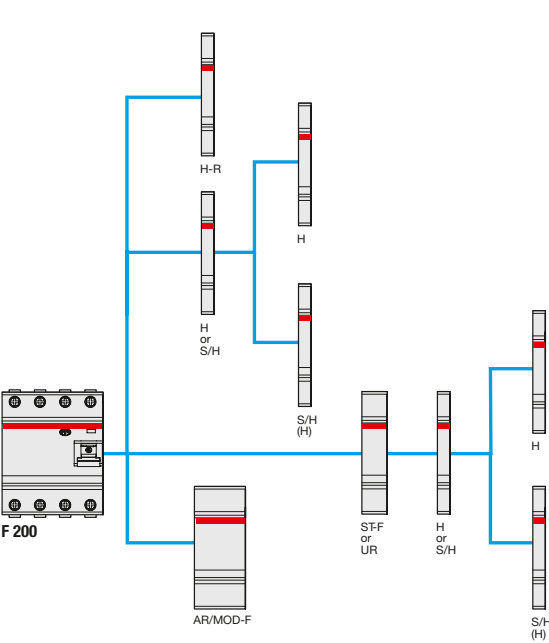
Combination of auxiliary elements with F200
