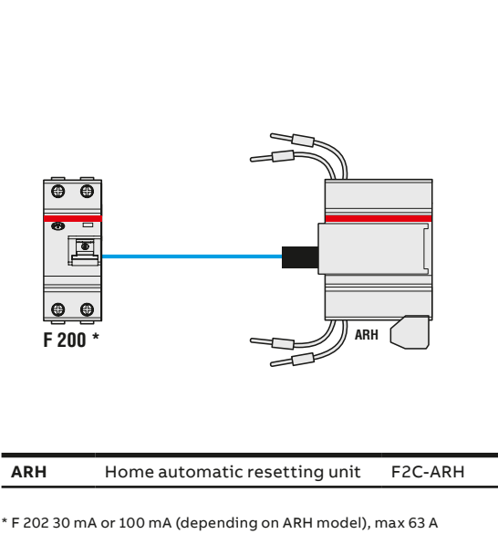
Combination of home automatic resetting unit with F200
