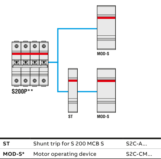
Combination of S200P with motor operating device
