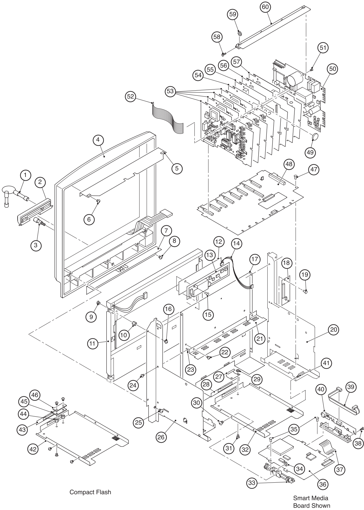
Figure 1 Identification of parts – chassis components
