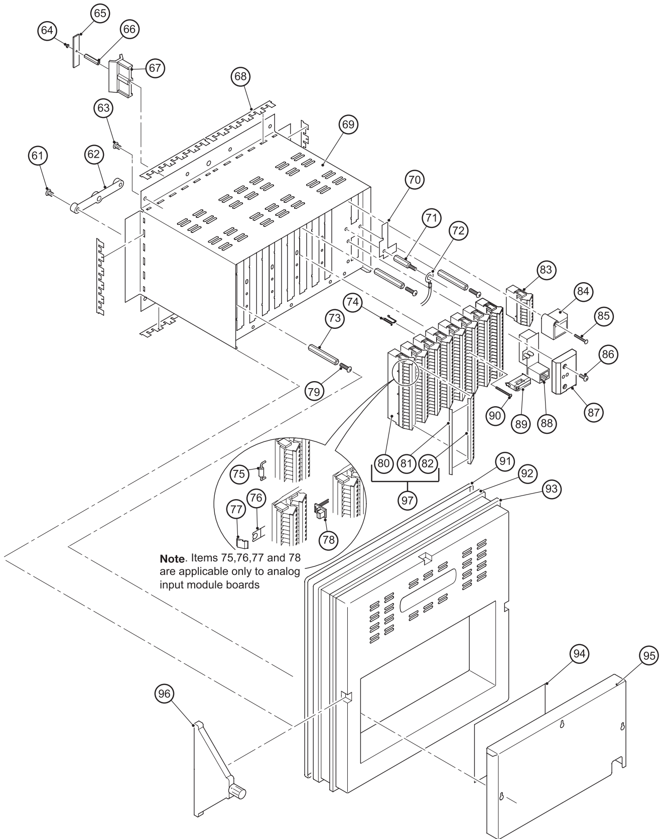
Figure 2 Identification of parts – instrument and chassis
