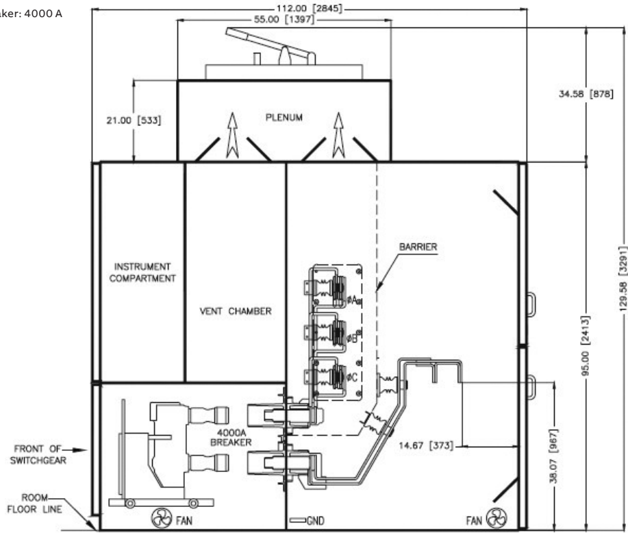
SIDE SECTION
