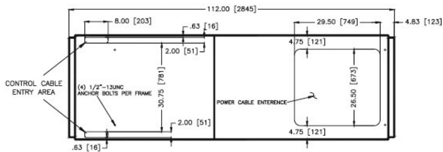
FLOOR PLAN
