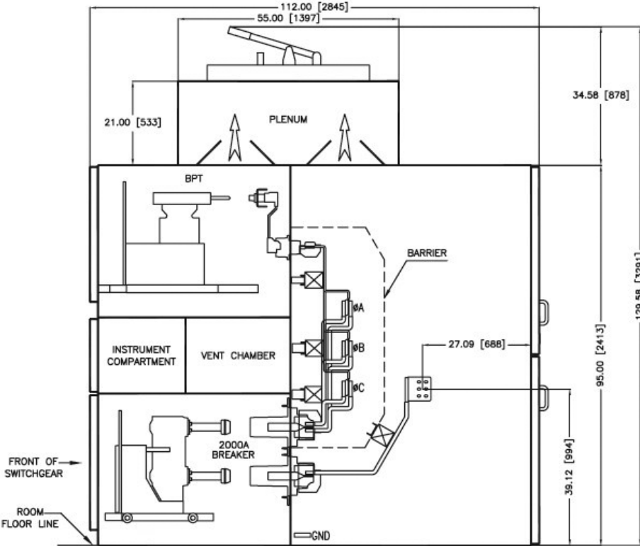
SIDE SECTION
