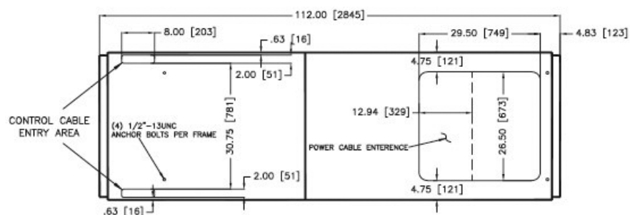
FLOOR PLAN
