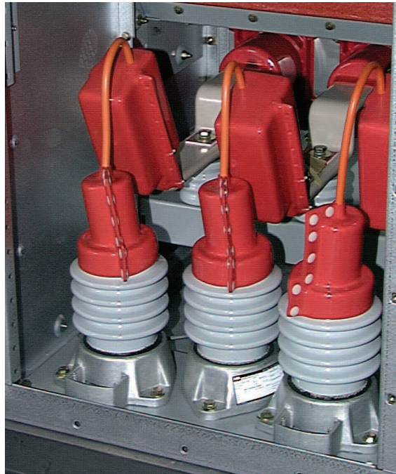
— 13 Large fixed-mount CPT up to 75 kVA 3-phase or 50 kVA single-phase
