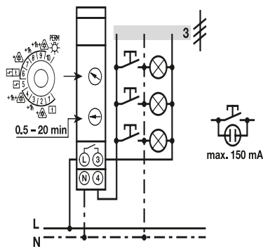
E 232E-230 Multi 10 3 conductor
