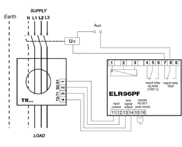
ELR96PF - undervoltage release wiring
