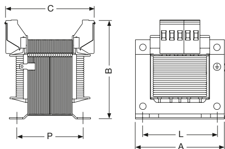
TM-C, TM-S and TM-I Control, Safety and Insulating transformers
