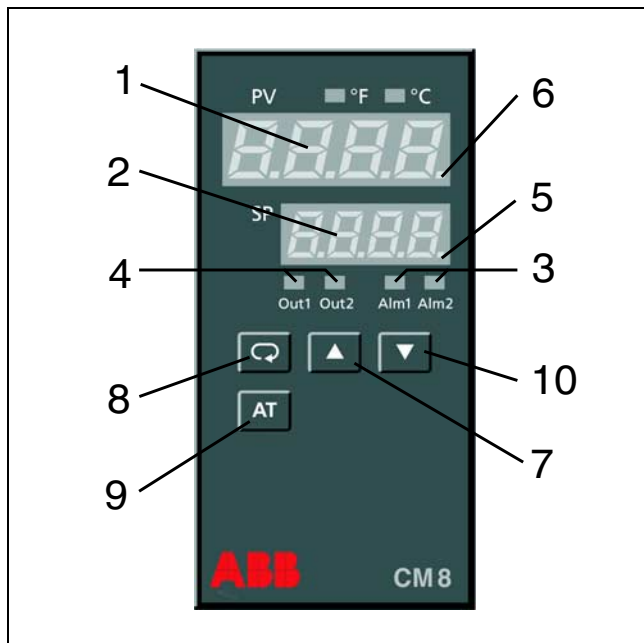
Fig. 3 Front panel Z-18793 1 Process variable 2 Setpoint 3 Status LED for alarm relay 4 Status LED for output relay 5 Status display „manual mode“ 6 Status display „selftune active“ 7 Key „increase“ 8 Key „menü“ 9 Key „start selftune“ or „back to main operator level“ 10 Key „decrease“
