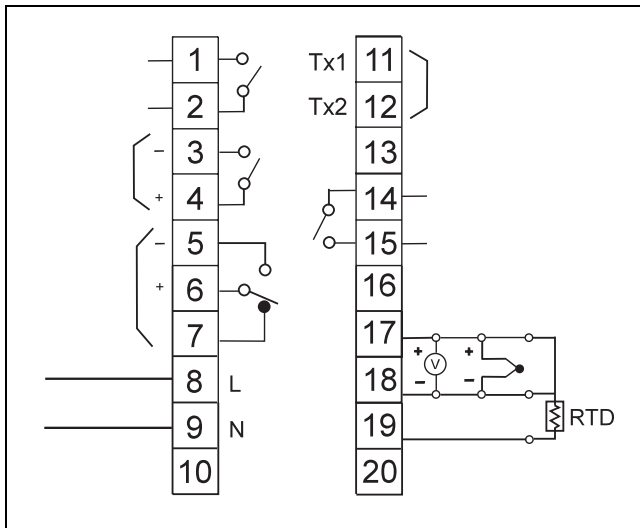
Fig. 2 Wiring diagram Z-18795 1, 2 Alarm 1 3, 4 Control output 2 5, 6, 7 Control output 1 8, 9 Power supply 11, 12 Retransmission of process variables 14, 15 Alarm 2 17, 18 19 Sensor input (RTD, TC, mA)
