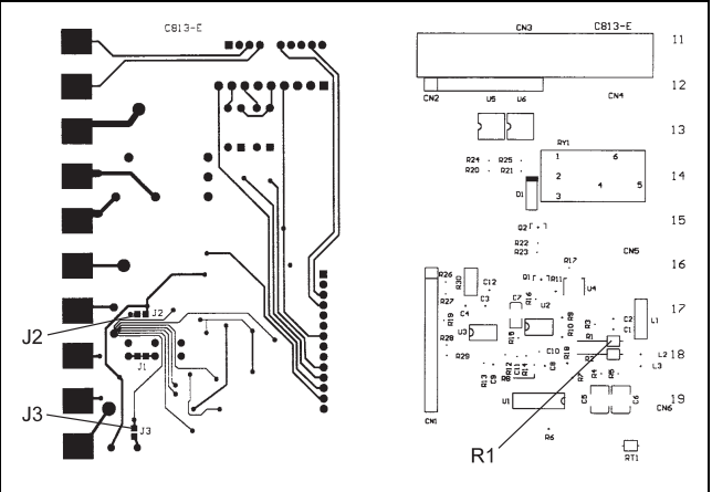
Bild 8 R1 resistor Z-18826 J2 soldered jumper J3 soldered jumper
