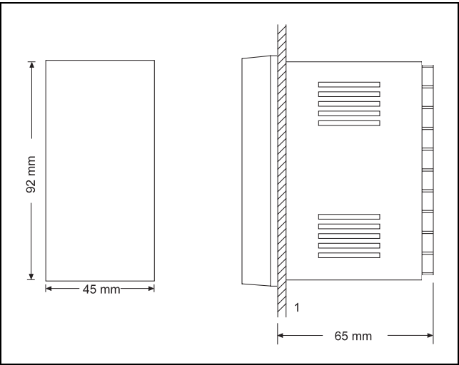
Fig. 1 Dimensional diagram Z-18794 left Panel cutout right Depth behind panel 1 Panel
