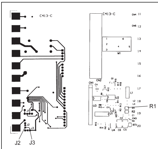
Bild 8 R1 resistor Z-18825 J2 solder jumper J3 solder jumper
