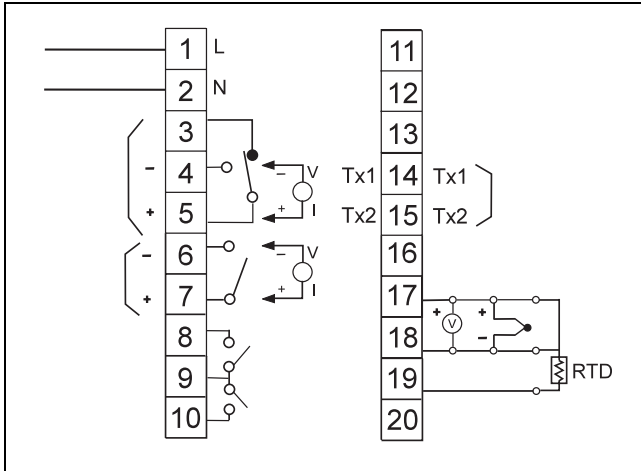
Fig. 7 Wiring diagram Z-18791 1, 2 Power supply 3, 4, 5 Control output 1 6, 7 Control output 2 8 Alarm 1 9 Alarm Com. 10 Alarm 2 14, 15 Retransmission of process variables 17, 18 19 Sensor input (RTD, TC, mA)
