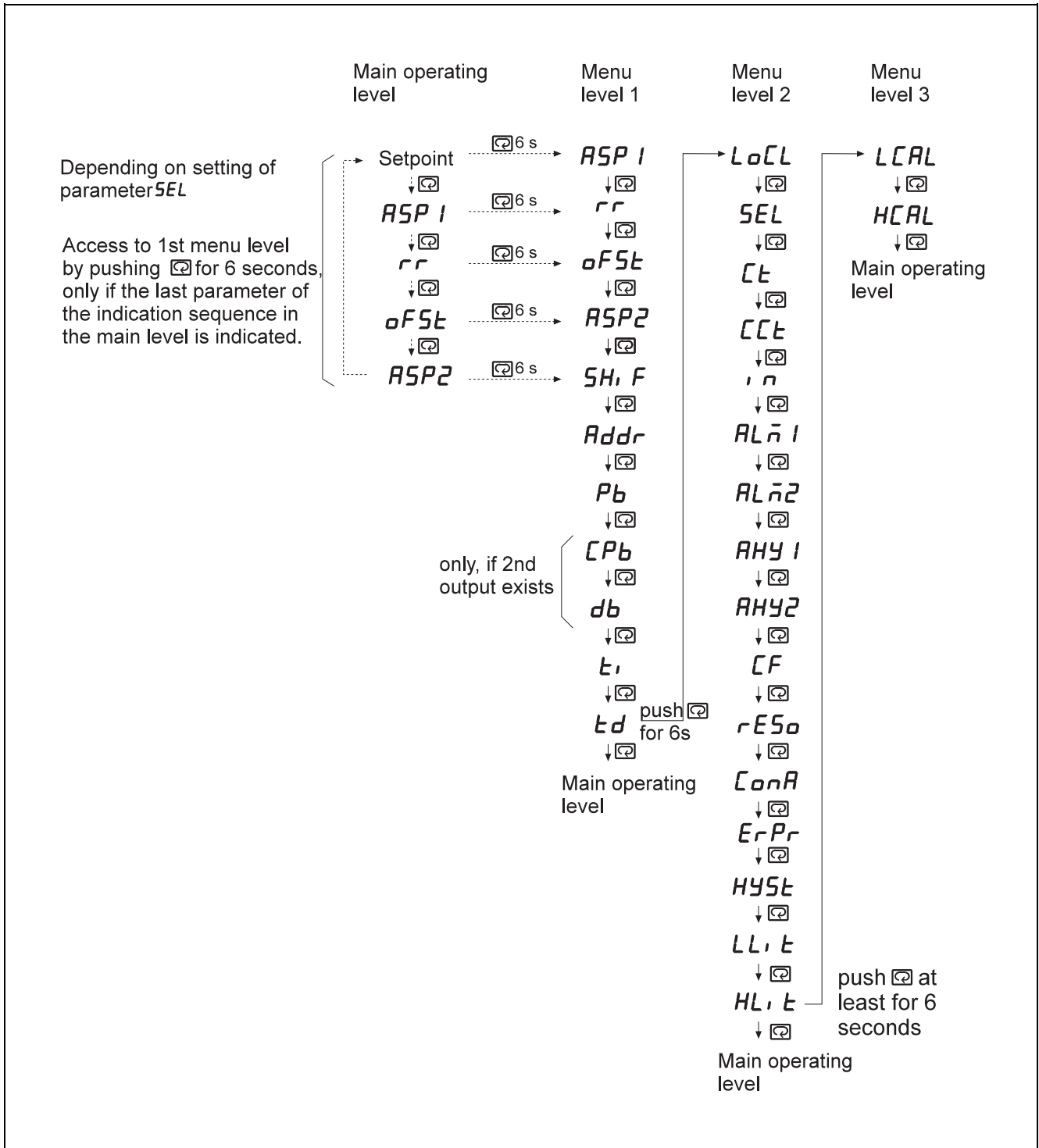
Fig. 4 Flow diagram Z-18891
