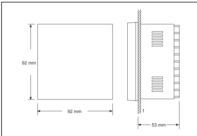
Fig. 1 Dimensional diagram Z-18790 left Panel cutout right Depth behind panel 1 Panel
