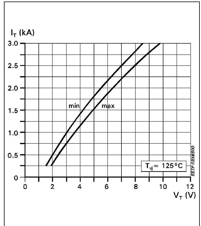
Fig. 3 On-state voltage characteristics T_{vj} = 125\text{ }^\circ\text{C} , 10 ms half sine
