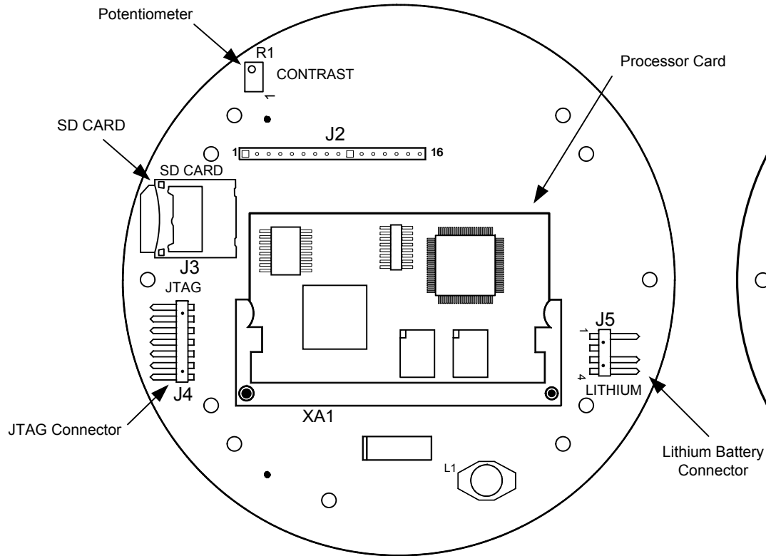
Motherboard Primary Component Side
