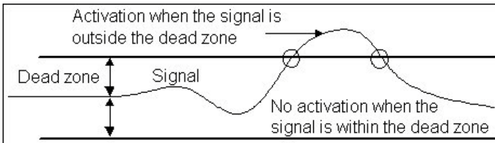
Figure 58. A dead zone on both sides of a desired signal value
