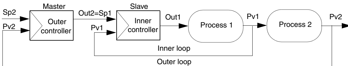
Figure 66. Illustration of two controller modules connected in cascade
