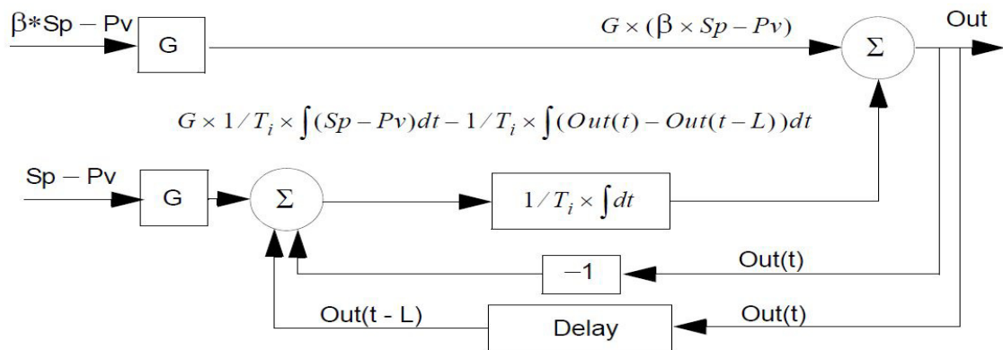
Figure 56. The principle of a PPI controller
