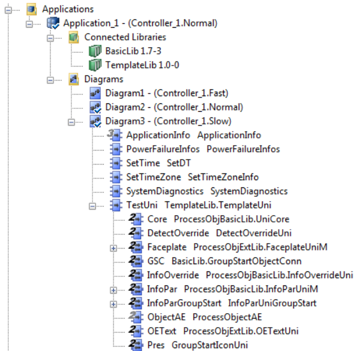
Figure 11. TemplateUni used in a diagram under the application
