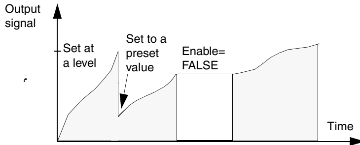
Figure 89. The integrator function sums the input signal ( In ) value over time
