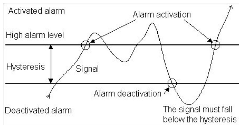
Figure 57. Activation is desired when a signal exceeds a high alarm level
