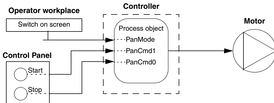
Figure 139. Control steps in Panel mode. This solution is recommended for large applications, where the PanMode parameter is connected to an operator workplace
