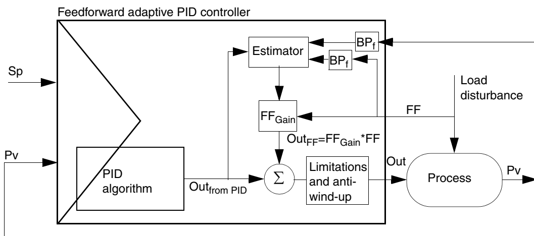
Figure 76. The principle of the feedforward adaptive PID controller
