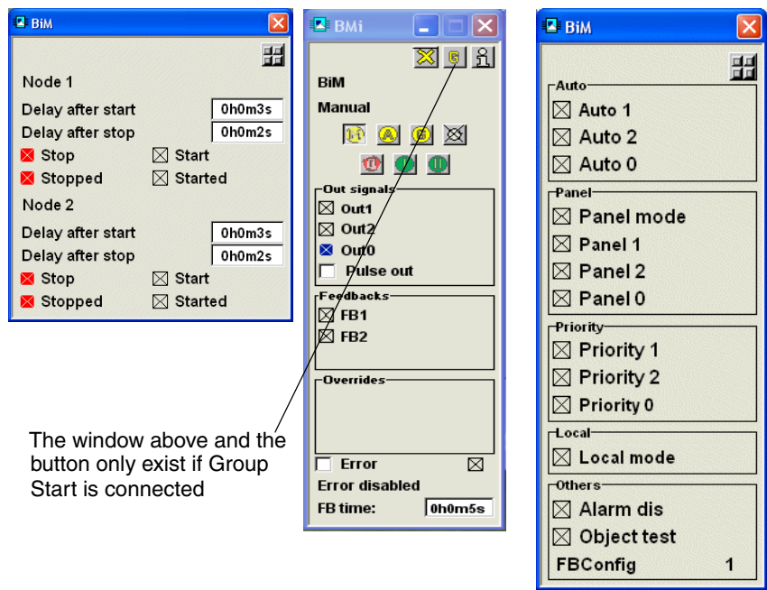
Figure 130. Control Builder interaction windows for Bi(M)
