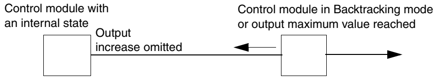
Figure 50. Example of when a succeeding control module has reached a limit value; the preceding control module stops further integration (anti-windup)
