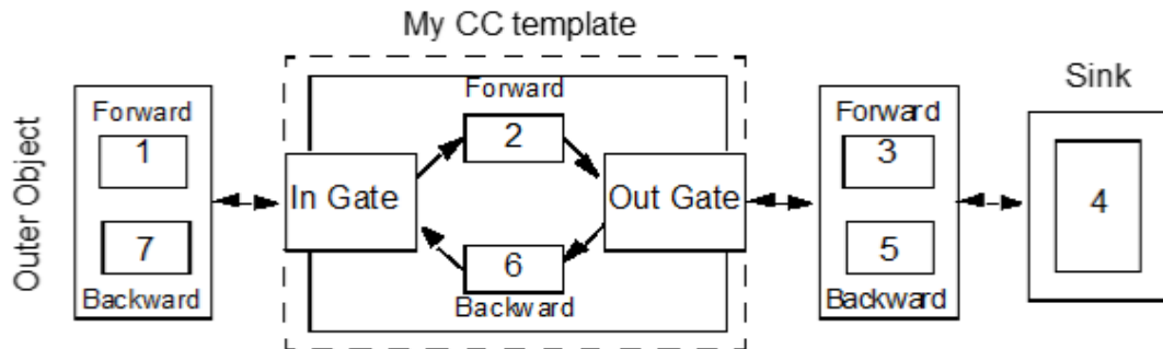
Figure 23. My CC template object is protected by the Gate modules on both sides to ensure a secure signal traffic with ControlConnection
