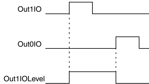
Figure 123. OutputIOLevel state diagram
