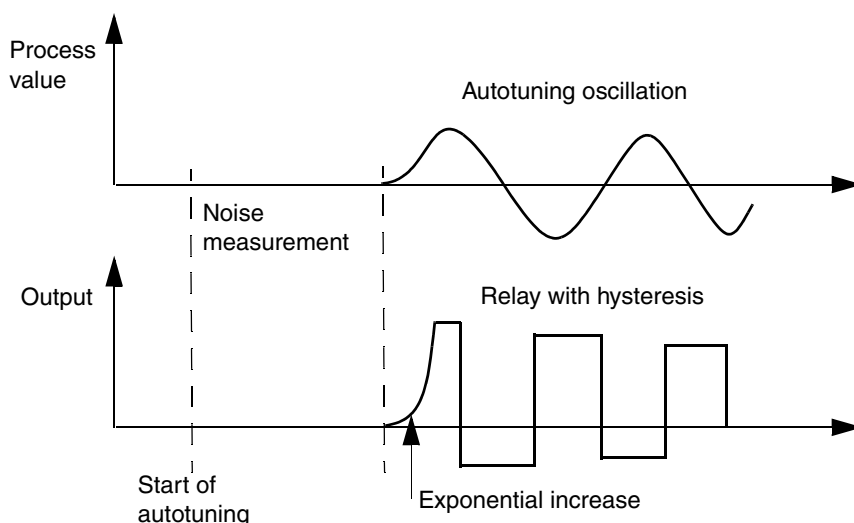
Figure 73. The process value oscillation
