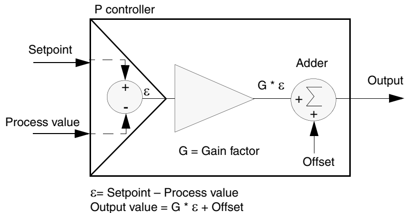
Figure 54. The basic P controller
