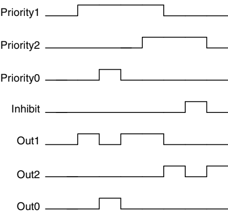
Figure 127. State diagram showing Priority command priorities and output signals with the effect of Inhibit
