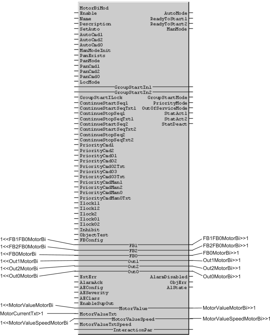
Figure 137. MotorBi function block with connections to variables
