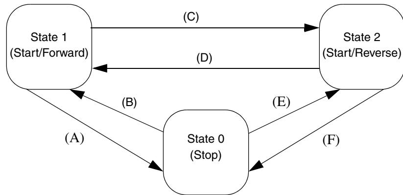
Figure 126. Manual maneuvers interlocking signals
