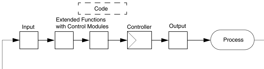
Figure 64. A control loop with all functions defined by control modules from the control libraries
