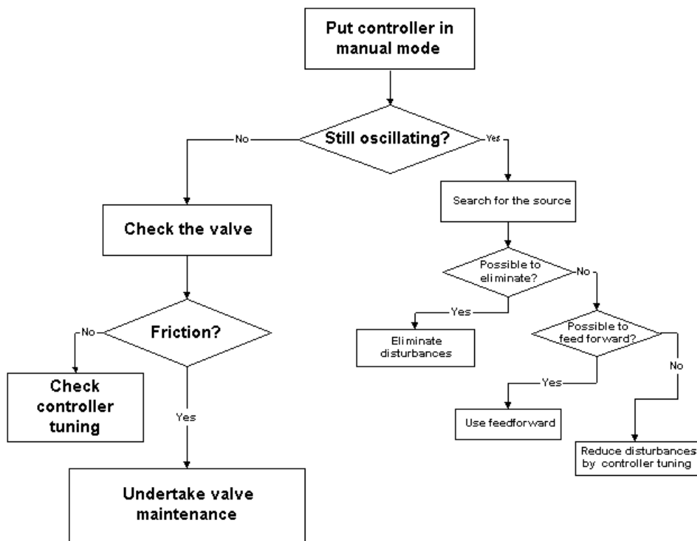
Figure 82. Flow chart for oscillation diagnosis
