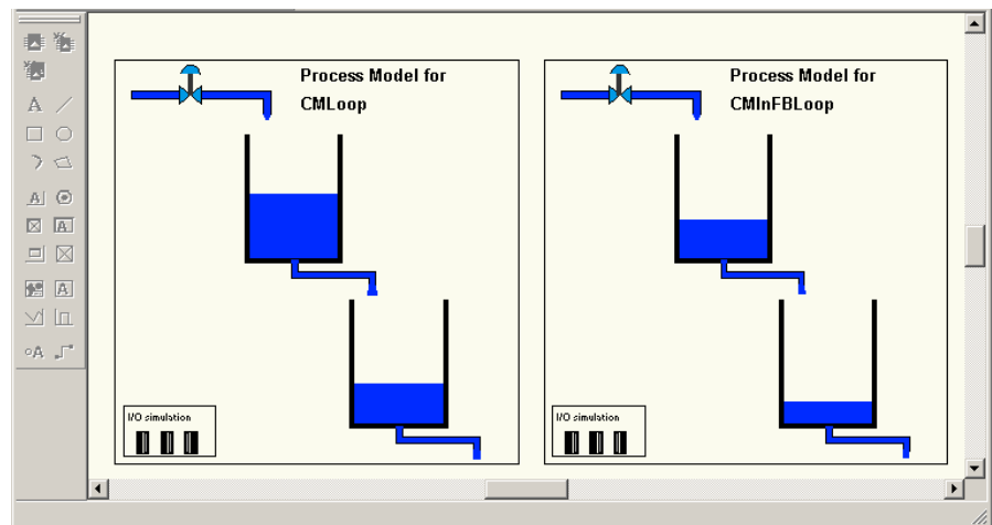
Figure 116. The Fuzzy Control Loop application in online mode showing two methods of programming
