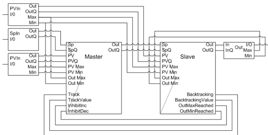
Figure 103. Example of a cascade control loop consisting of function blocks, with signal ranges added
