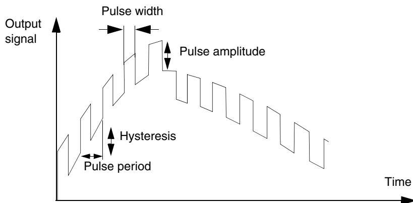
Figure 83. The stiction compensator signal is superimposed on the analog output signal
