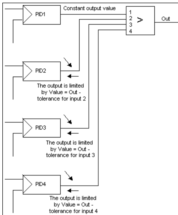
Figure 105. Example of a Max4CC control module with inputs from controller outputs
