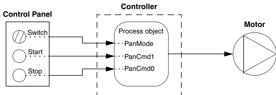
Figure 138. Control steps in Panel mode. This solution is recommended for small applications, where all three panel parameters are connected from a control panel
