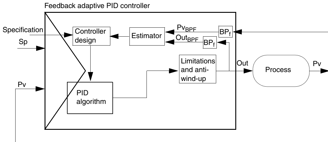
Figure 75. The principle of the feedback adaptive PID controller
