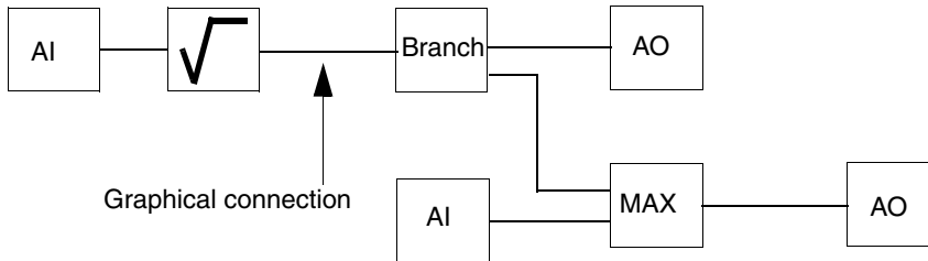
Figure 48. A chain of connected control modules for analog signal handling
