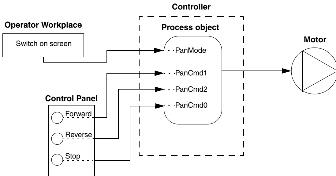
Figure 141. The Panel mode control diagram. A general solution for large applications, where the PanMode parameter is connected to an operator workplace
