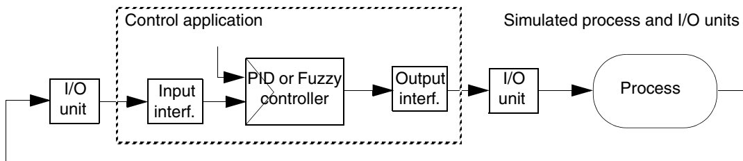
Figure 111. The principle for control applications, the simulated processes and I/O units
