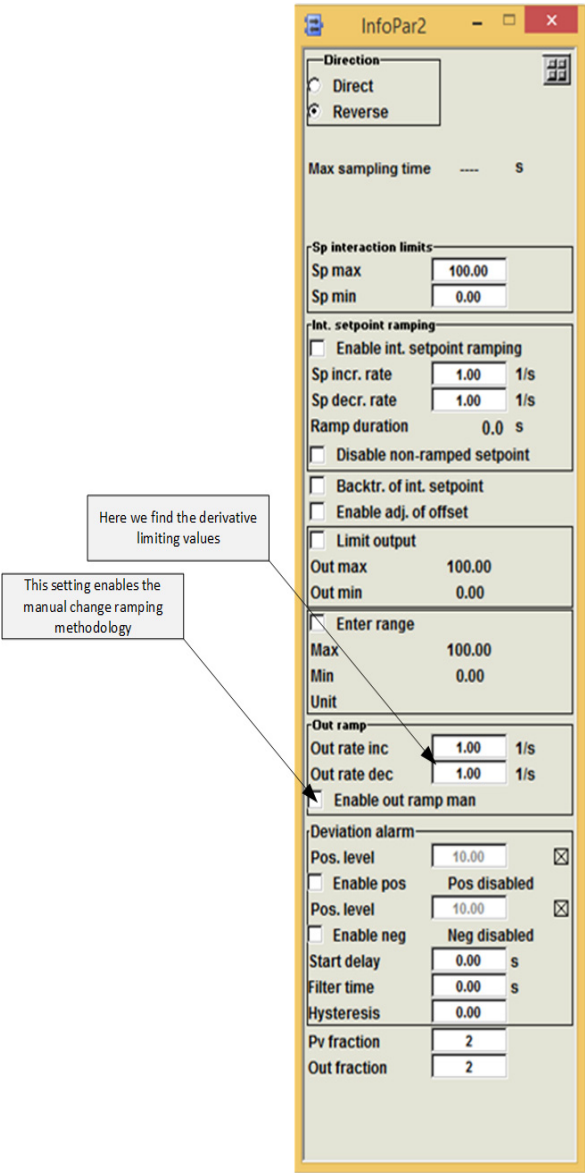
Figure 59. The interaction window of a PidCC or PidAdvancedCC
