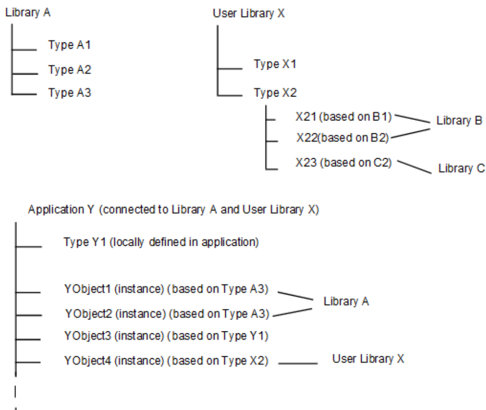
Figure 7. Building complex solutions based on standard libraries, self-defined libraries, and locally defined types
