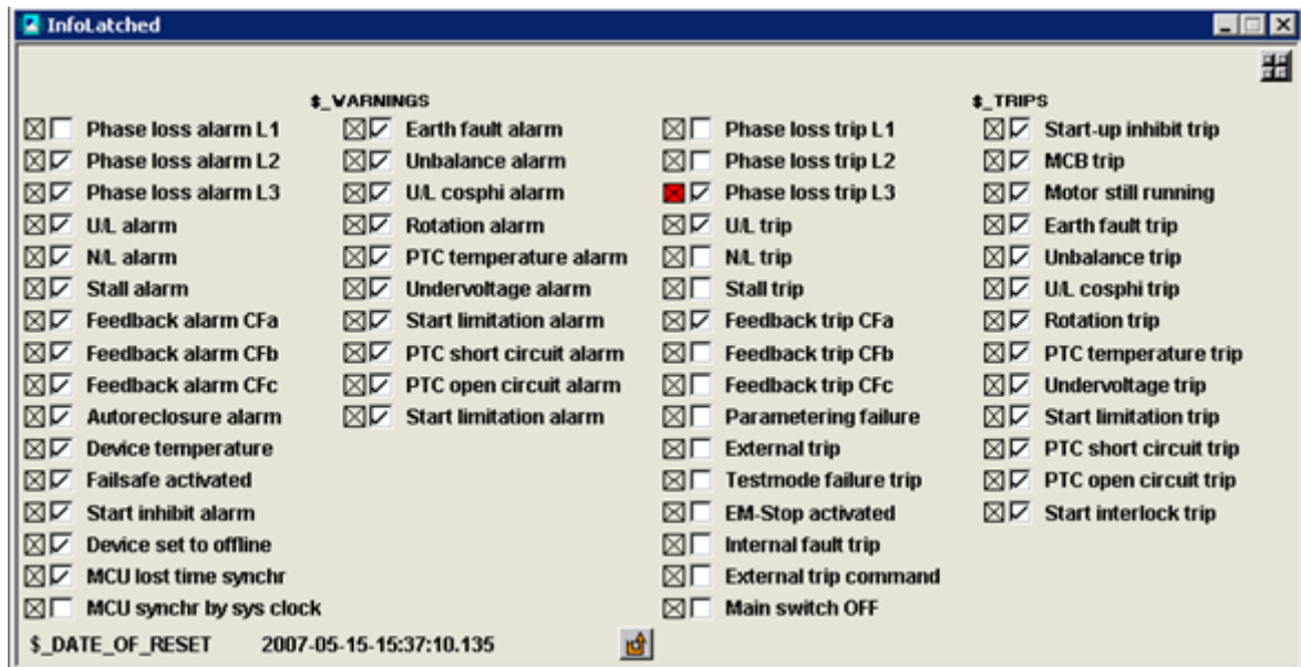
Figure 147. MCUExtended Main Interaction Window- Alarm Indication
