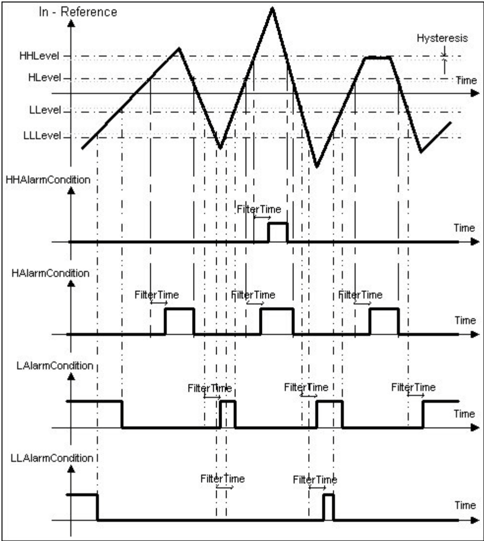
Figure 110. Level Detection example
