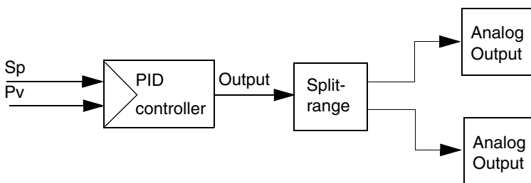
Figure 69. Example of split-range control where the output range from the controller is divided into two branches with different ranges
