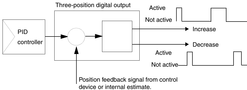
Figure 80. The principle of the three-position digital output function
