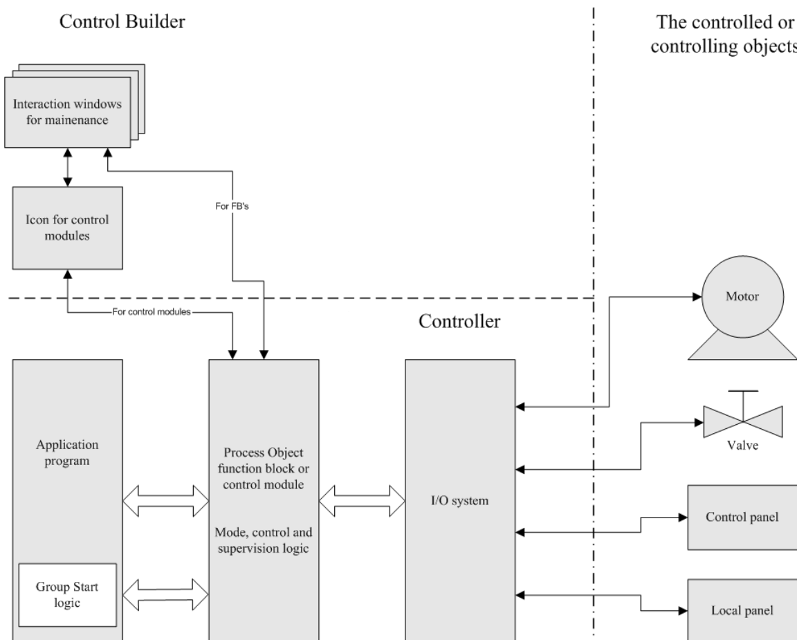
Figure 118. Relations between a function block or control module and the remote objects
