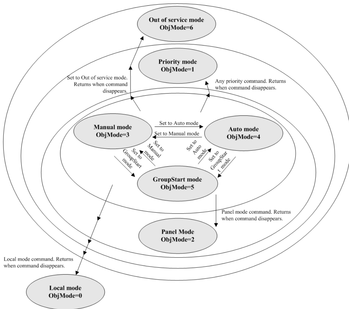
Figure 120. Core object modes and their relationship
