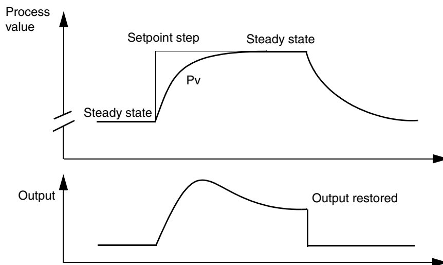
Figure 74. Setpoint step identification and output restoration
