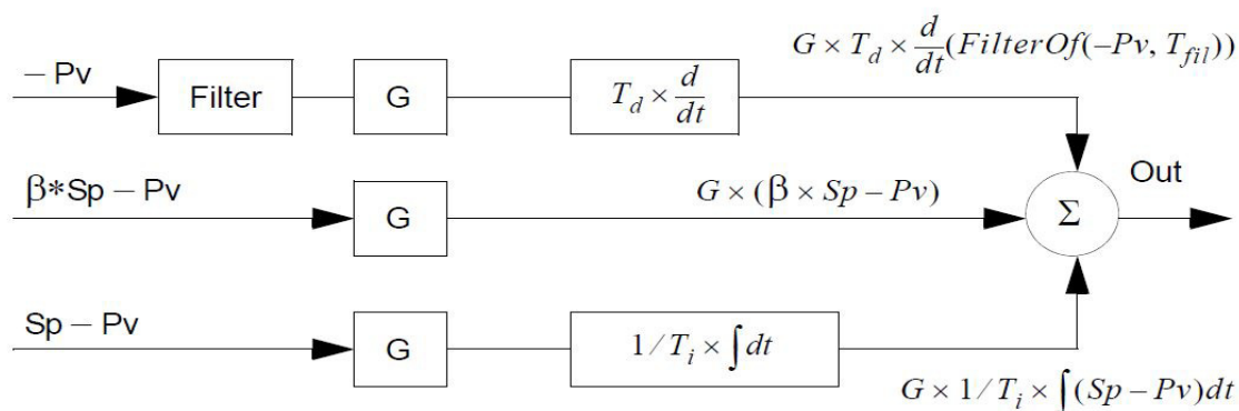
Figure 55. The principle of an ideal PID controller
