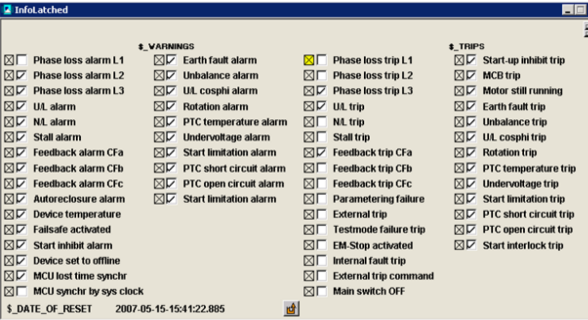
Figure 146. MCUExtended Main Interaction Window - Trips
