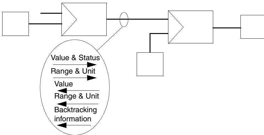
Figure 51. A graphical connection of ControlConnection type with its main signal flow forward and a flow backward
