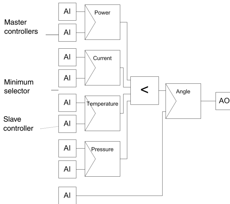
Figure 106. Example using control modules for override control in a heat pump using a minimum selector control module
