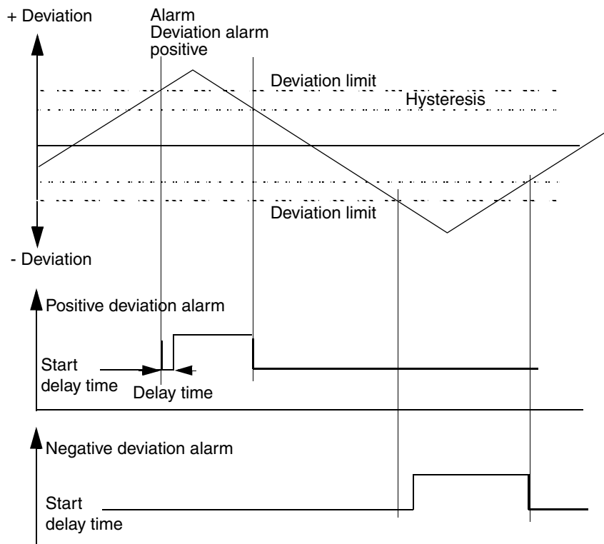
Figure 70. Overview of the controller deviation alarm limits
