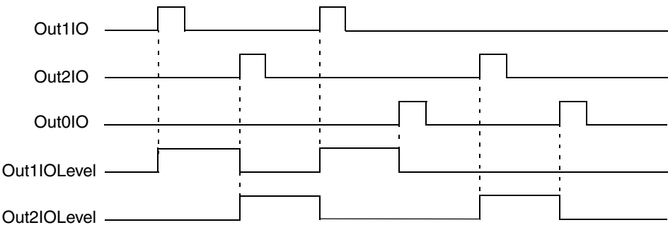
Figure 128. OutputIOLevel state diagram
