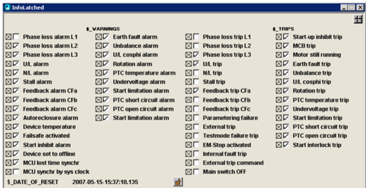
Figure 145. MCUExtended Main Interaction Window- Alarms
