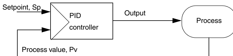
Figure 53. A control loop with the function block of a PID controller
