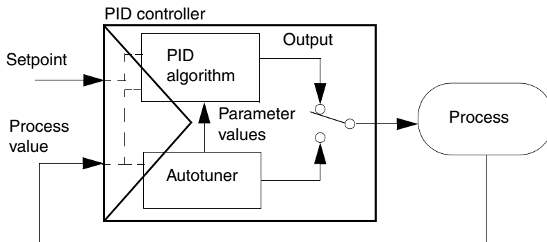
Figure 72. The principle of autotuning in a PID controller with the Autotuner function
