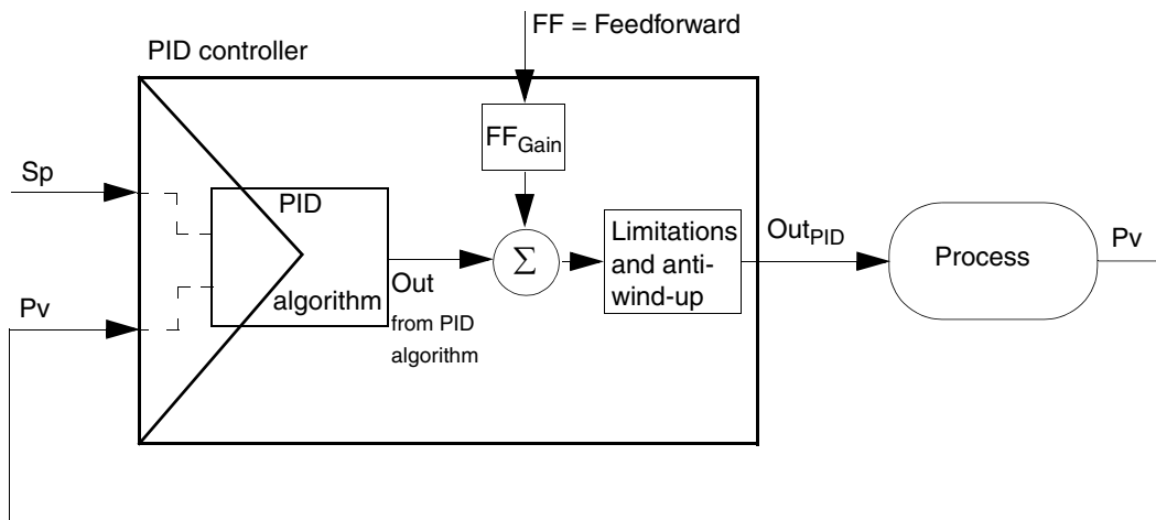
Figure 71. The feedforward principle in the controller
