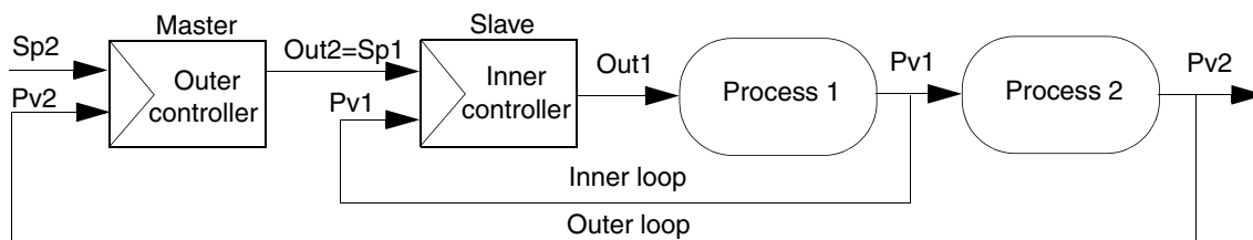
Figure 115. Illustration of two PID function blocks or controller modules connected in cascade
