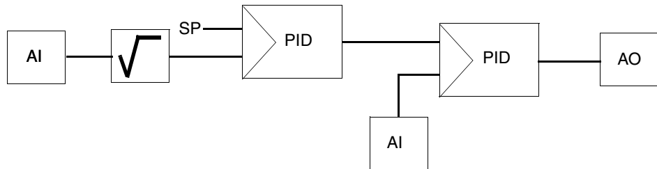
Figure 47. Example of graphical connections between control modules making a control loop
