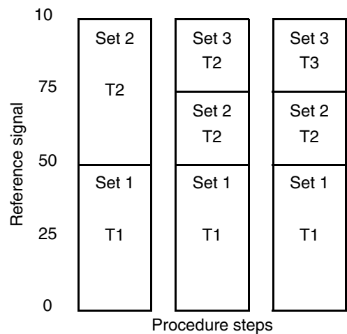
Figure 78. Example of the procedure for gain scheduling in three sets
