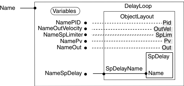
Figure 98. The result of DelayLoop parameter and variable connections
