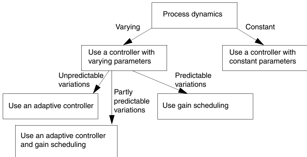
Figure 79. Procedure used to decide which controller to use, adaptive control and/or gain scheduling
