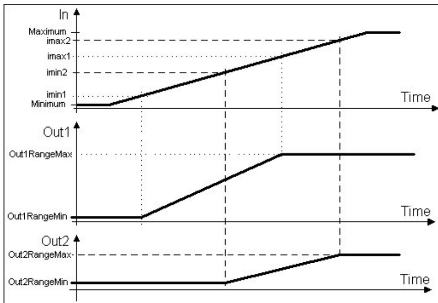
Figure 107. Split range
