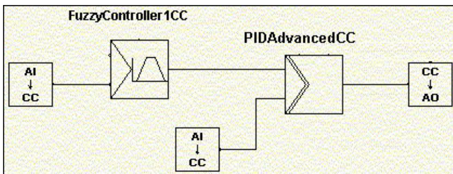
Figure 62. Fuzzy control relations
