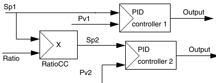
Figure 68. Example of ratio controllers where the setpoint from the first controller is multiplied by a factor to obtain the setpoint for the second controller
