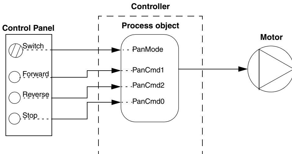
Figure 140. The Panel mode control diagram. A general solution for smaller applications, where all four Panel parameters are connected from a control panel
