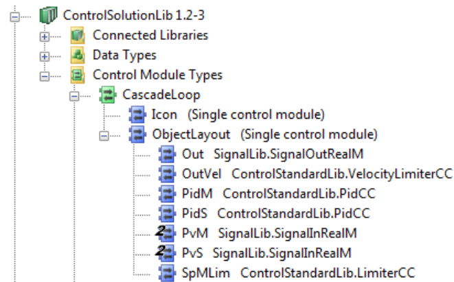
Figure 91. Standard types in a control loop solution (CascadeLoop)
