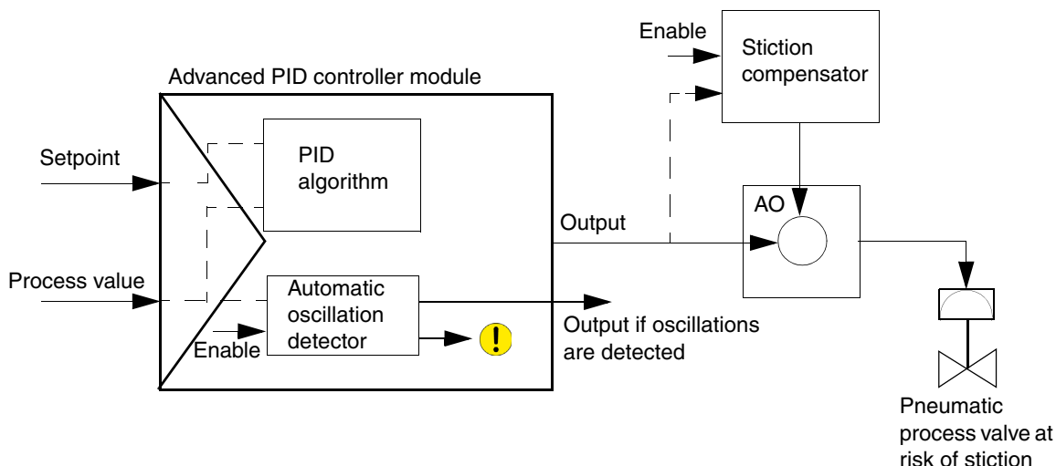
Figure 81. Principles for detecting and solving friction problems
