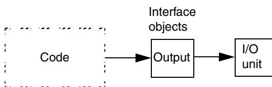
Figure 88. Handling of output signals
