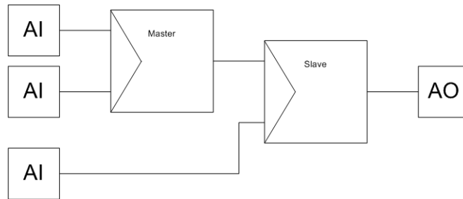
Figure 104. Example of a cascade control loop consisting of control modules
