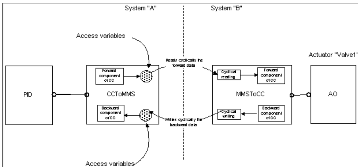
Figure 52. ControlConnection using control modules
