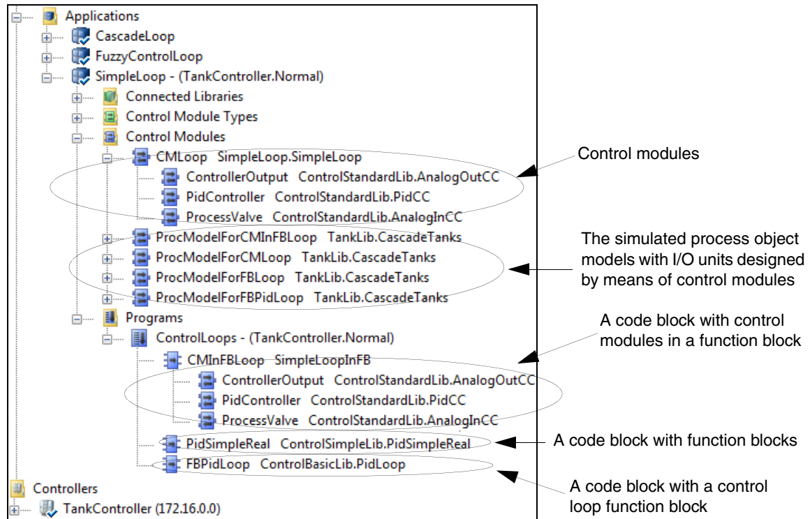
Figure 112. The four methods of designing an application and the simulated process
