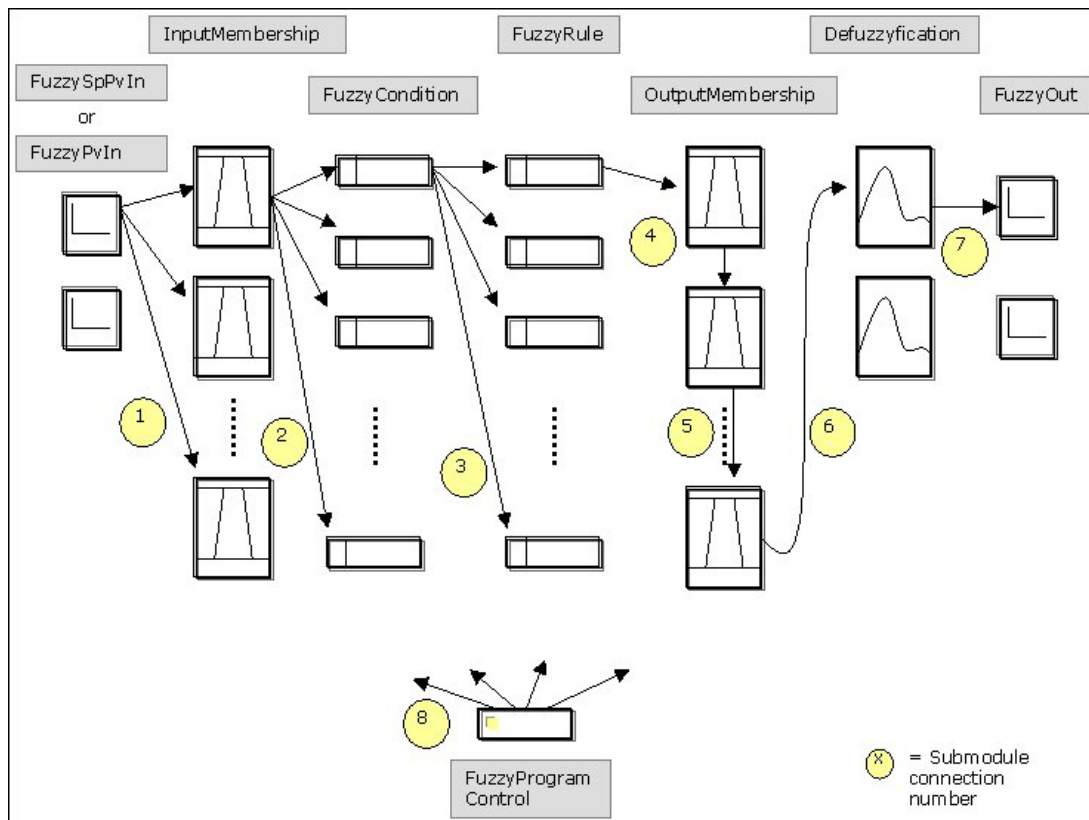
Figure 63. Sub-module connections in the fuzzy controller templates
