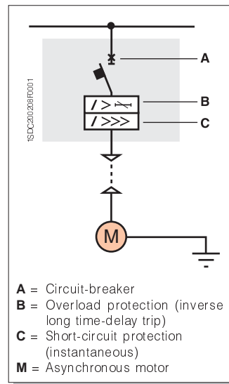
Diagram showing direct starting of an asynchronous motor using just the circuit-breaker fitted with an electronic overcurrent release.
