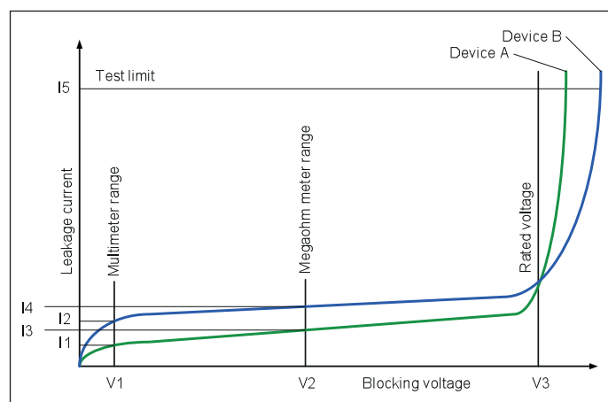
Figure 1: Comparison of blocking characteristics of two semiconductor devices of the same type.
