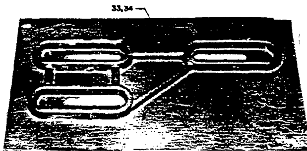
Fig. 10 Bus support, molded
