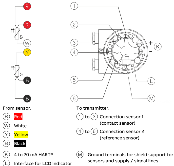
Figure 17: Pin assignment for processing and displaying component.
