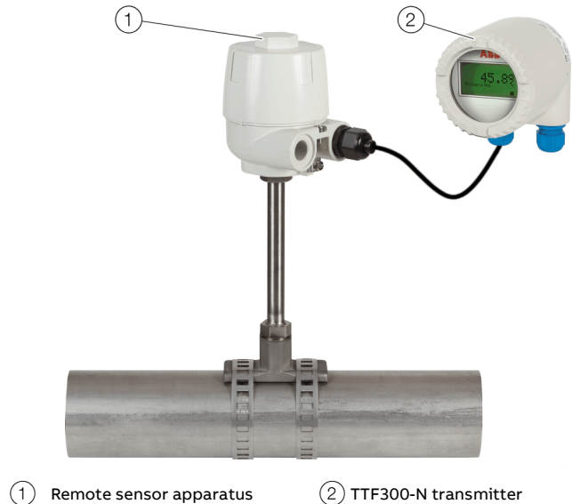
Figure 11: Example of installing TTF300-N with TSP341-N remote sensor apparatus
