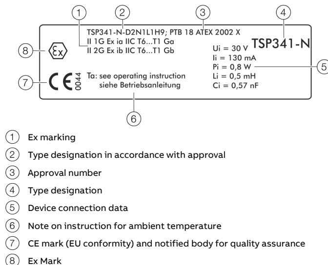
Figure 9: Additional certification plate for devices with type of protection "Ex i - intrinsic safety" (example)
