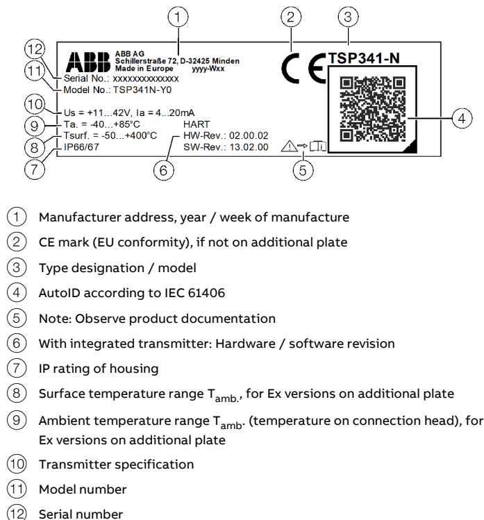
Figure 8: TSP341-N name plate (example for 'Ex i - intrinsic safety' type of protection)
