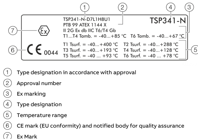
Figure 10: Additional certification plate for devices with type of protection "Ex d - flameproof enclosure" (example)
