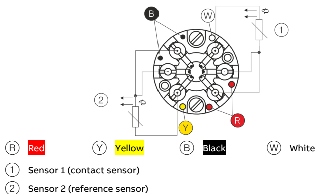
Figure 16: Pin assignment for ceramic terminal block of measuring component (view from above)
