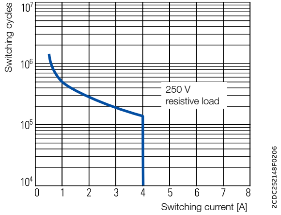
Contact lifetime
