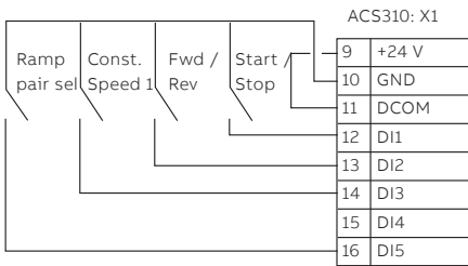
DI configuration NPN connected (sink)
