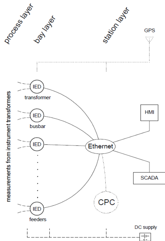
Fig. 1. Schematic of the Block-layer reliability technique adjusted to secondary substation systems connected to the process level (left) and to adjacent substations (right). Time-synchronization sources (GPS) and DC supplies are parallel components, crossing several layers, consequently they are not included to any layer.
