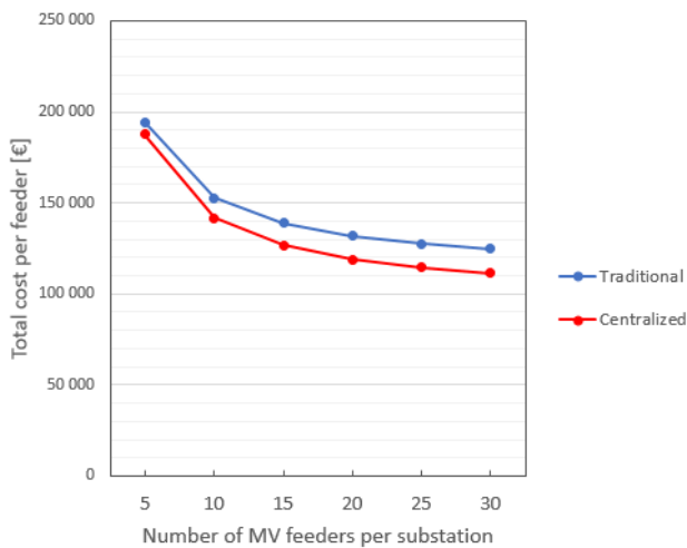
Fig. 4. The normalized total cost of the secondary system per MV feeder in traditional and centralized architectures for substations.
