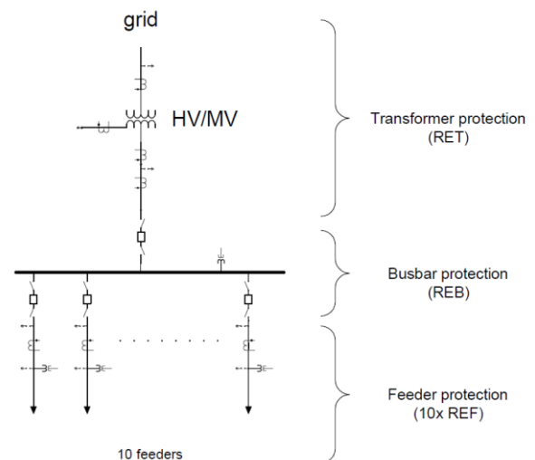
Fig. 3. The diagram details the test substation with its one transformer bay (RET relay), ten feeder bays (REF relay) and a busbar bay (REB relay).
