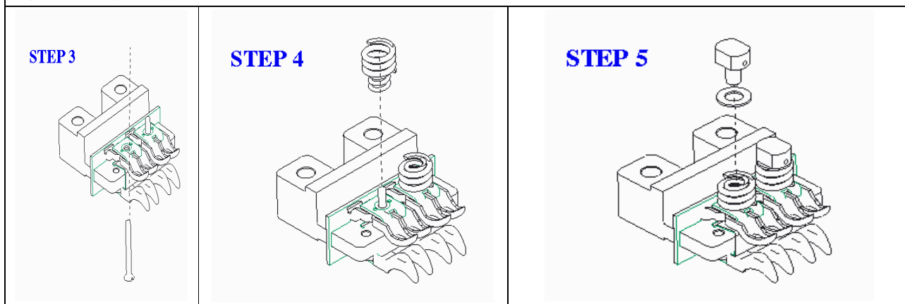
Figure 25. Steps in Exploded Views (WPS-32/WPH-32/WPX-32)
