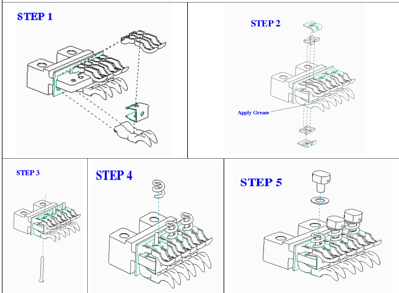
Figure 26. Steps in Exploded Views (A WPS-40/ WPX-40/WPS-50/WPX-50 )
