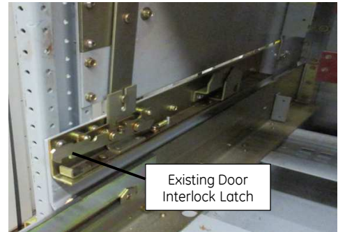
Figure 30B. AKD-10—Door Interlocking Components for WPS-32/WPH-32/WPX-32/WPS-40/ WPX-40/WPS-50/ WPX-50 Breaker.
