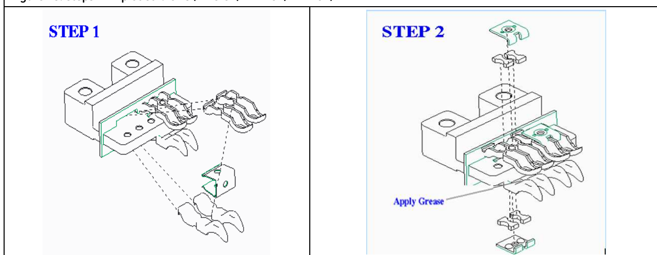
Figure 25. Steps in Exploded Views (WPS-32/WPH-32/WPX-32)
