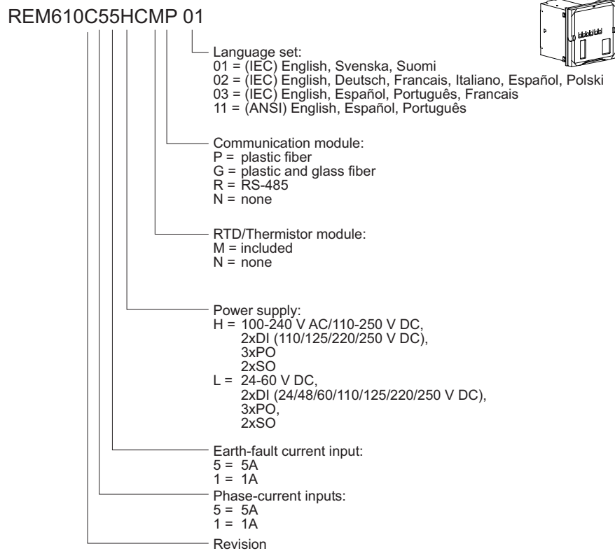
Fig. 7.-1 Ordering key for complete relays
