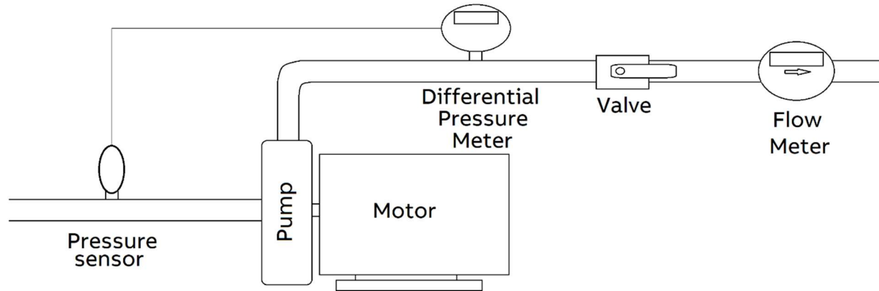
Figure 1: Lab setup
