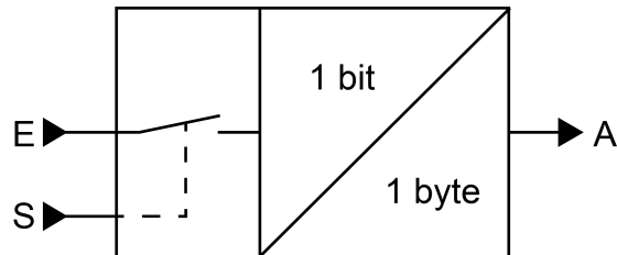
Image 23: Converter (1 bit -> 1 byte)
