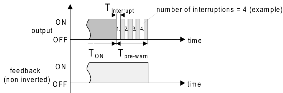
Image 5: The pre-warning function of the staircase function (example)
