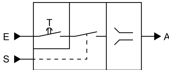
Image 24: Disabling element [Filtering/Time]
