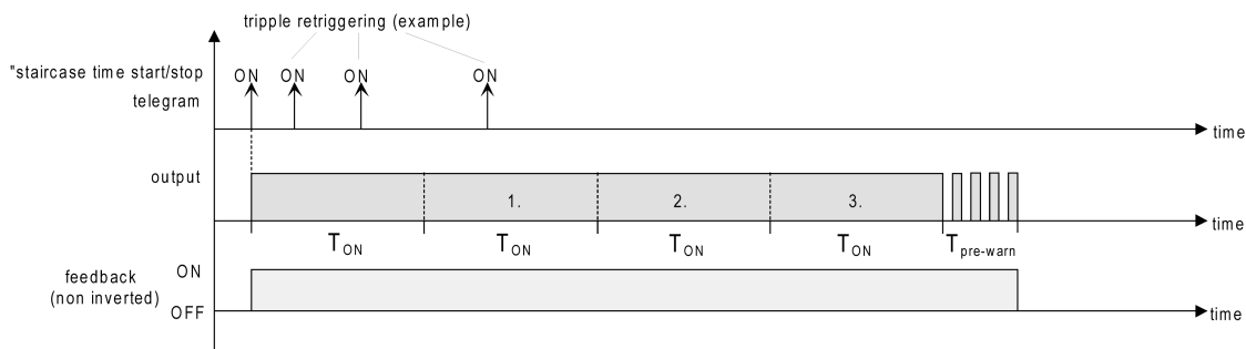
Image 6: Time extension of the staircase function
