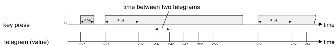
Image 15: Example of value adjustment without value range overflow
