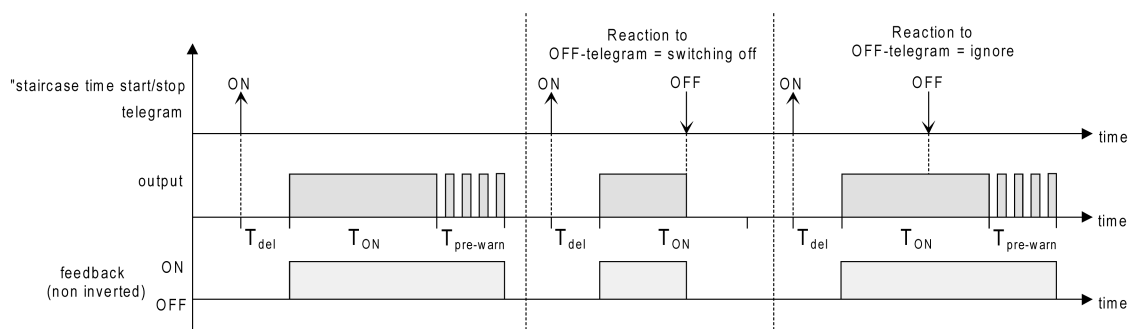
Image 4: Switch-off behaviour of the staircase function
