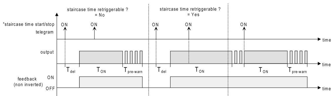
Image 3: Switch-on behaviour of the staircase function
