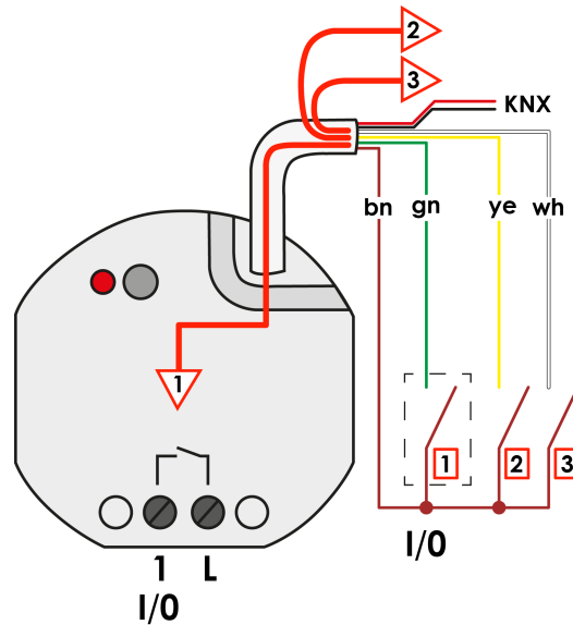
Image 9: Functionality of the input 1 when controlling the internal switching output as single-area operation
