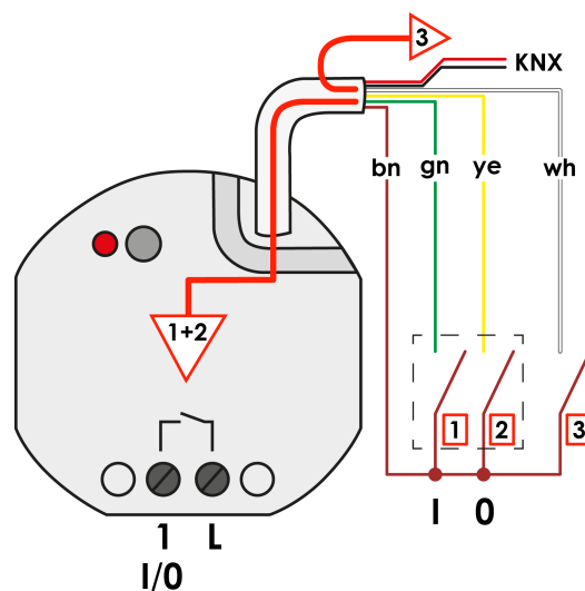
Image 10: Functionality of the inputs when controlling the internal Switching output as dual-area operation
