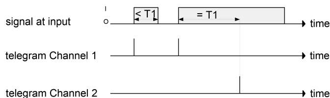
Image 22: Example for operation concept "Channel 1 and channel 2"
