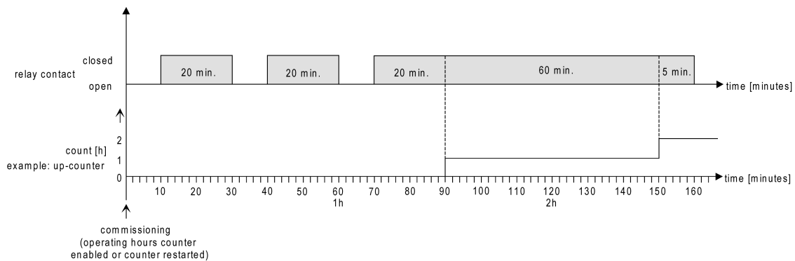
Image 8: Function of the operating hours counter (using the example of counted hours)
