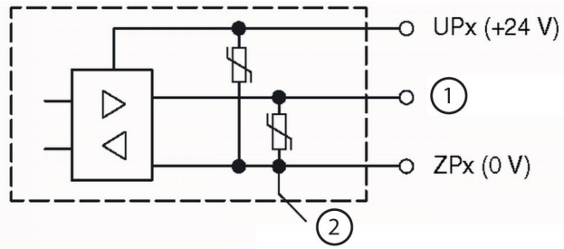
Fig. 1: Circuitry of a digital input/output with the varistors for demagnetization when inductive loads are switched off
