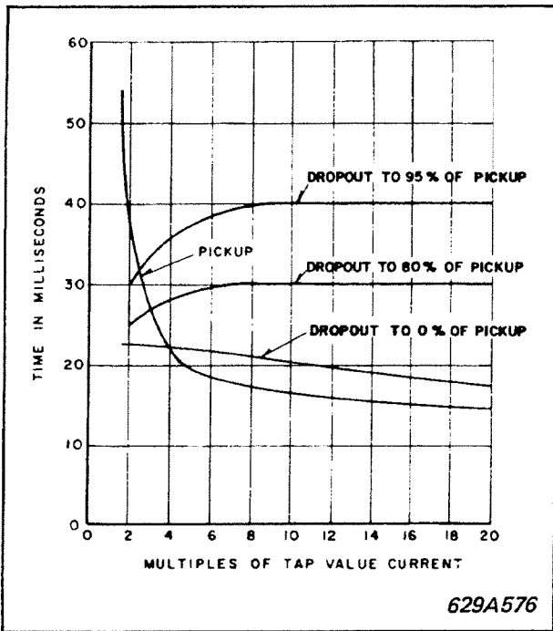
Fig. 6. Maximum Pick-Up and Drop-Out Time Curves for the Phase and Ground Overcurrent Units
