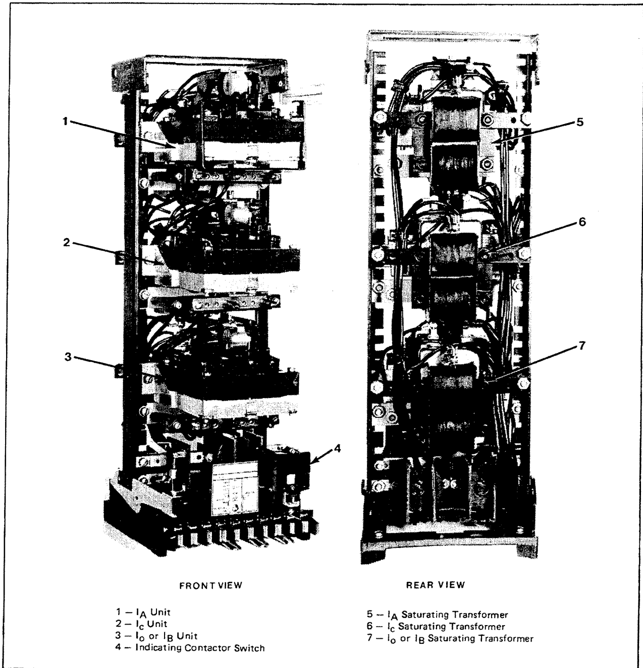
Fig. 1. Type KC-4 Relay Without Case.
