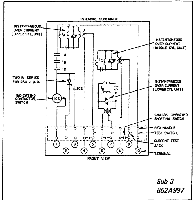
Fig. 9. Internal Schematic of the KC-4 Relay with Series Make Contacts in FT-41 Case.
