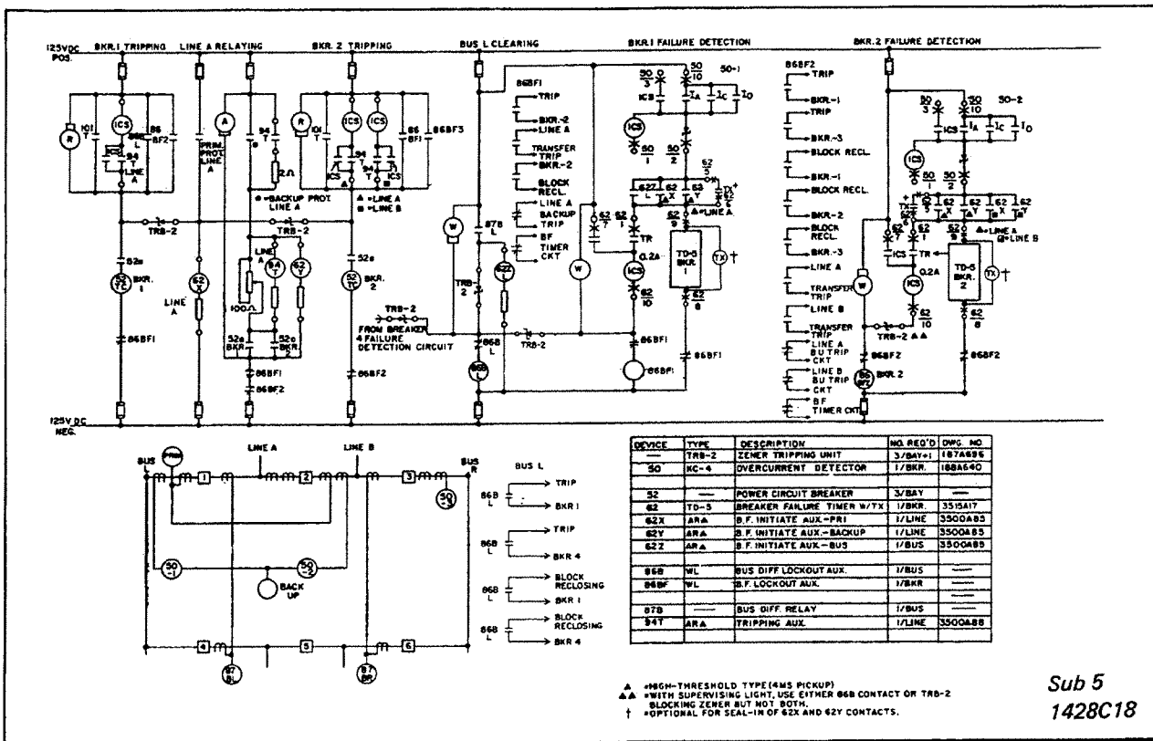
Fig. 4. External Connections for the KC-4 Relay – Breaker Failure Protection of a Breaker-and-a-Half Bus Arrangement – One Timer per Breaker.
