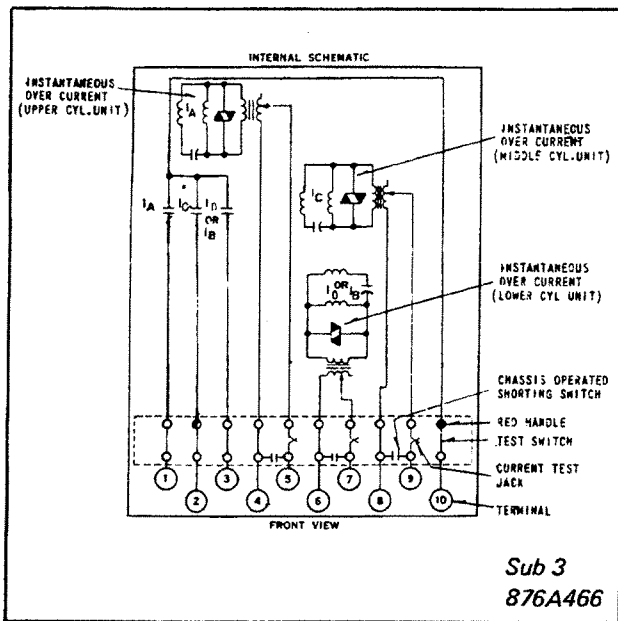
★ Fig. 10. Internal Schematic of the KC-4 Relay with one side of Contacts to Separate Terminals in FT-41 Case.
