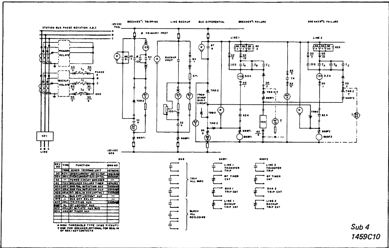
Fig. 2. External Connections for the KC-4 Relay – Breaker Failure Protection of a Single Bus/Single Breaker Arrangement – One Timer per Bus.
