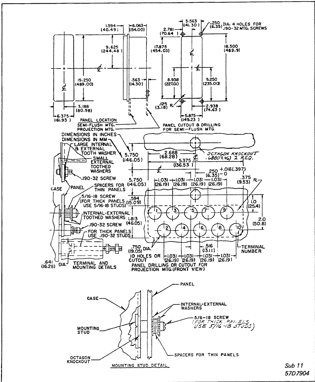
• Fig. 12. Outline and Drilling Plan for the KC-4 Relay in FT-41 Case.
