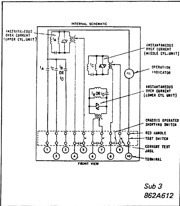
Fig. 8. Internal Schematic of the KC-4 Relay with Operation Indicator and Contacts to separate terminals in FT-41 case.
