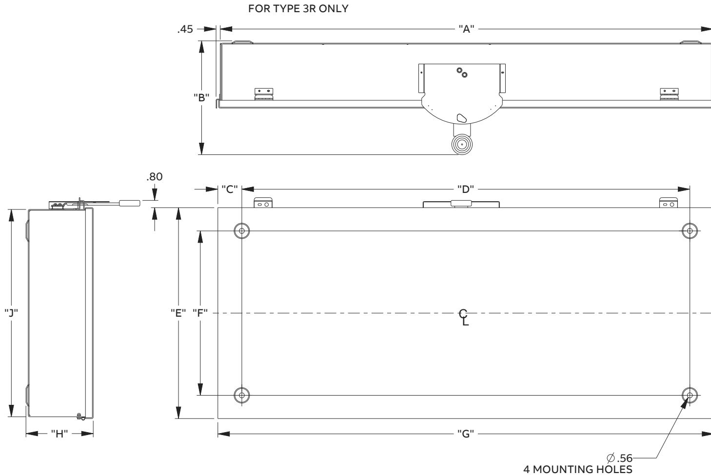
DIMENSION TABLE
