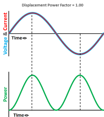
Figure 2 Power factor 1
