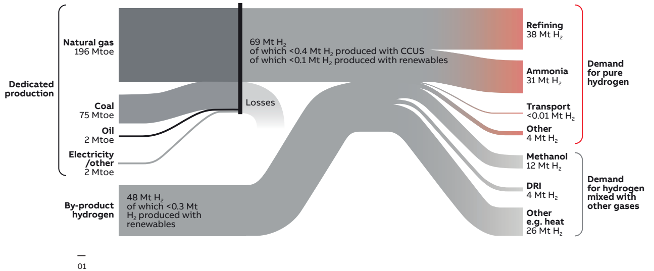
01 Value chains of today's global hydrogen industry (source: International Energy Agency)
