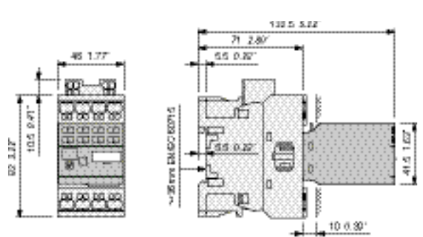
NF22EK, NF31EK, NF40EK + TEF4S electronic timer
