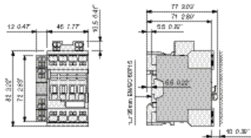
AF09..K, AF12..K, AF16..K+ CA4..K 1-pole auxiliary contact block
