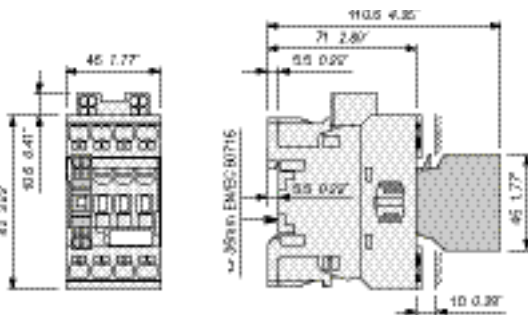
NF22EK, NF31EK, NF40EK + CA4..K 1-pole auxiliary contact block
