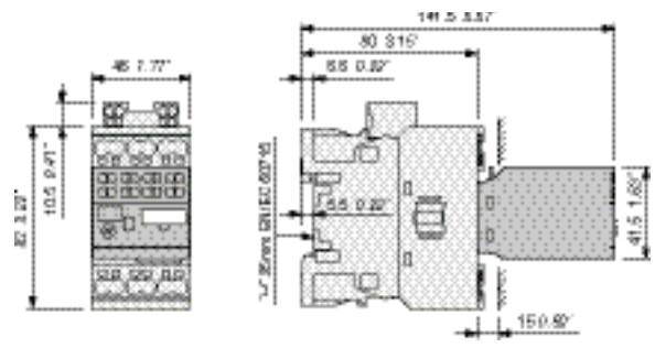
AF26..K, AF30..K, AF38..K + TEF4S electronic timer
