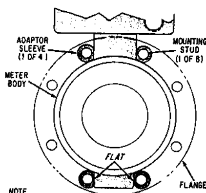
8-BOLT FLANGE PATTERN (ADAPTOR SLEEVE, TYPE II)
