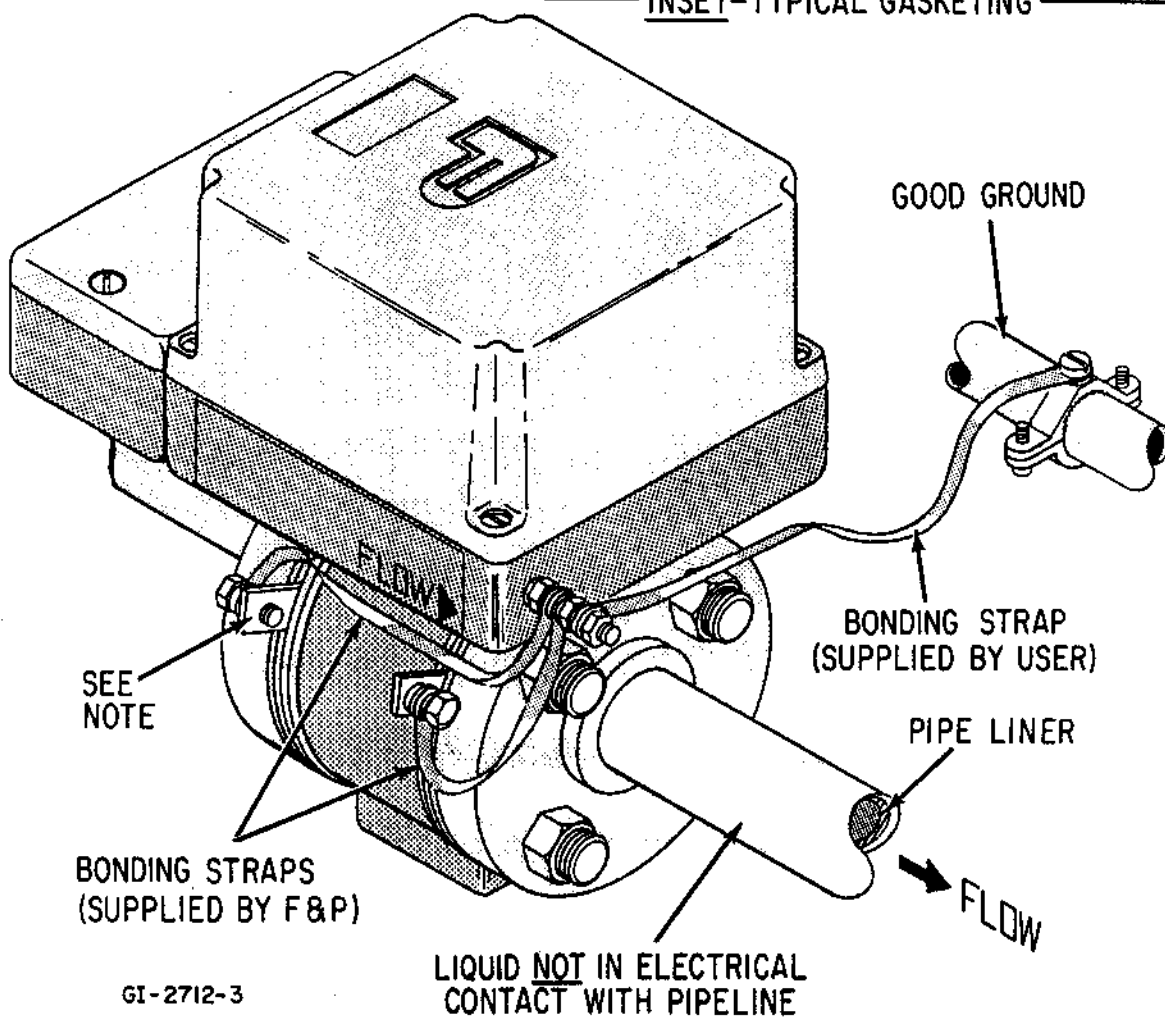
FIGURE 2-11. GROUNDING PROCEDURE, INSULATED PIPE
