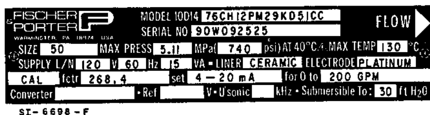
FIGURE 3-1. TYPICAL INSTRUMENT TAG
