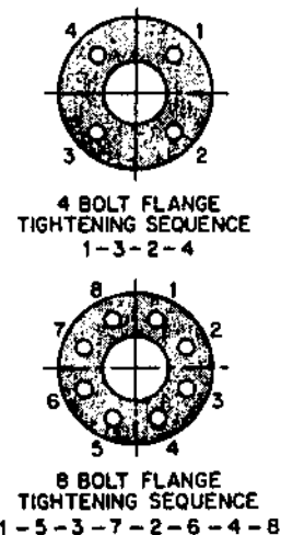
FIGURE 2-8. TYPICAL MOUNTING DIAGRAM, SANITARY FITTINGS
