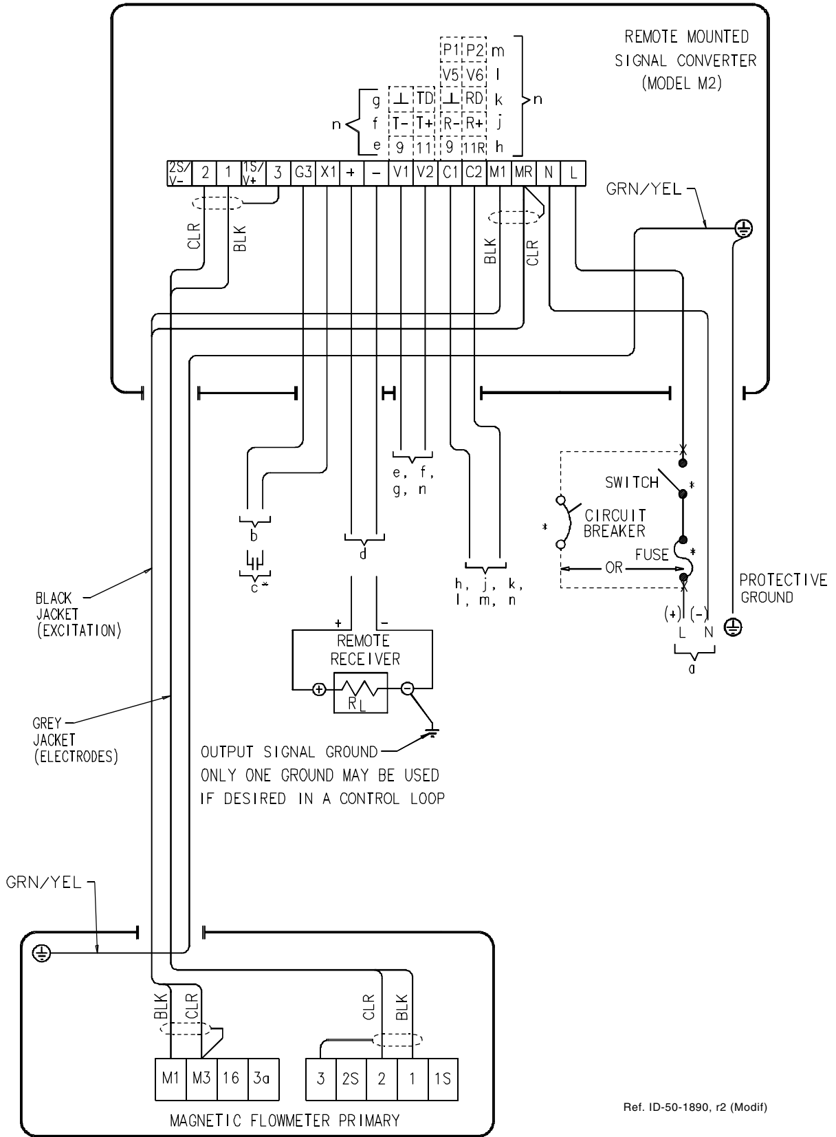
FIGURE 2-10. INTERCONNECTION DIAGRAM, MODEL 10DX3111G
