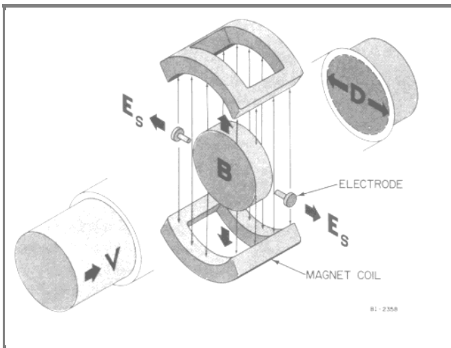
FIGURE 4-1. BASIC OPERATING PRINCIPLE
