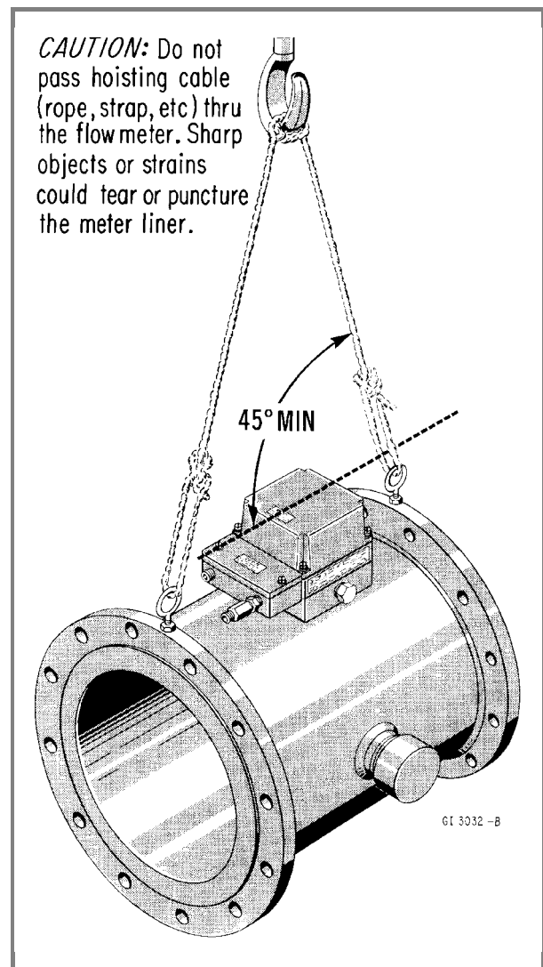
FIGURE 2-1. PROPER HOISTING TECHNIQUE
