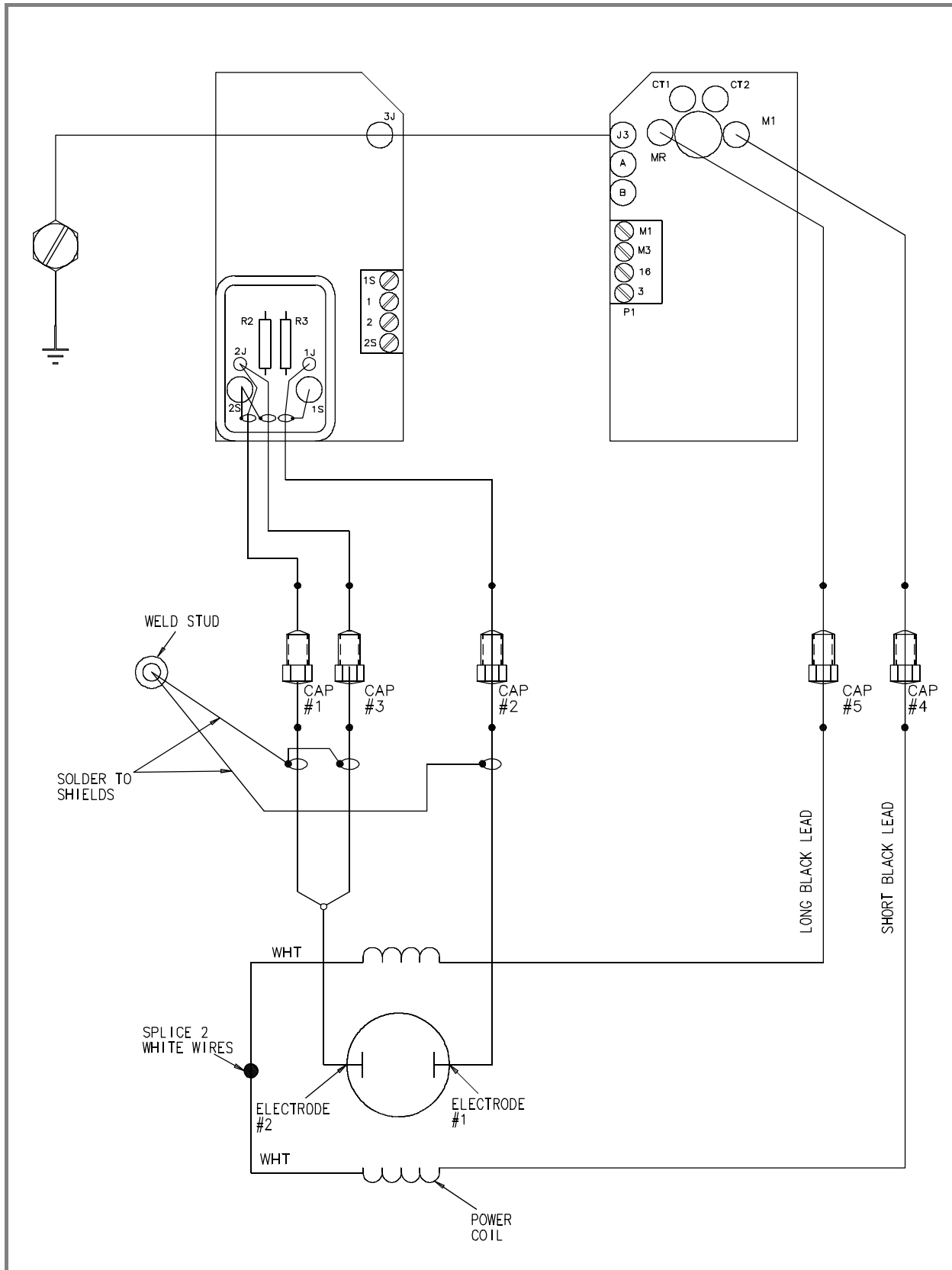
FIGURE 5-3. INTERNAL WIRING DIAGRAM, MODEL 10DX3111G
