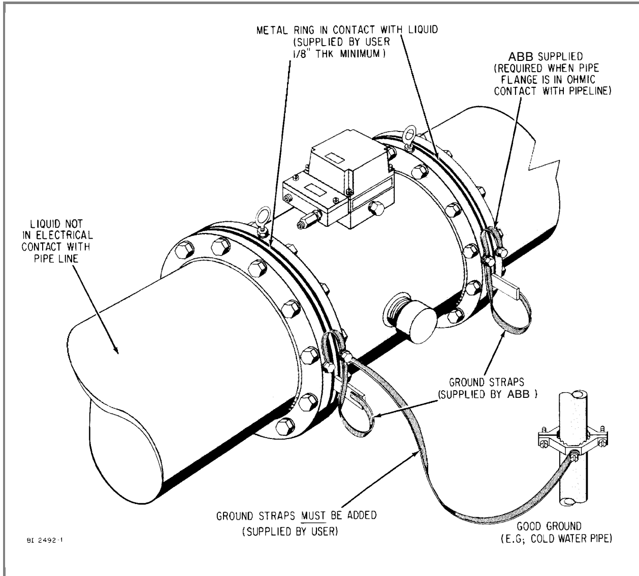
FIGURE 2-6. GROUNDING PROCEDURE; INSULATED PIPELINE
