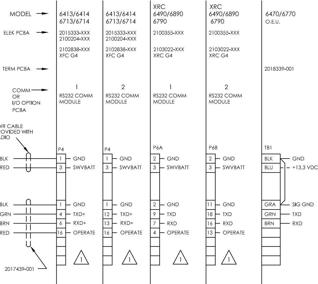
WIRING DIAGRAM INTEGRA-H 900 (SPREAD SPECTRUM) DATARADIO
