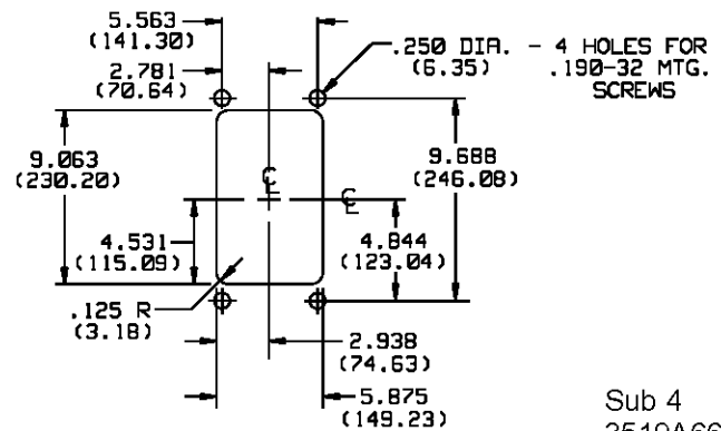
Figure 25: Outline and Drilling plan for the Type COM relay in the FT21 Case for Class 1E.
