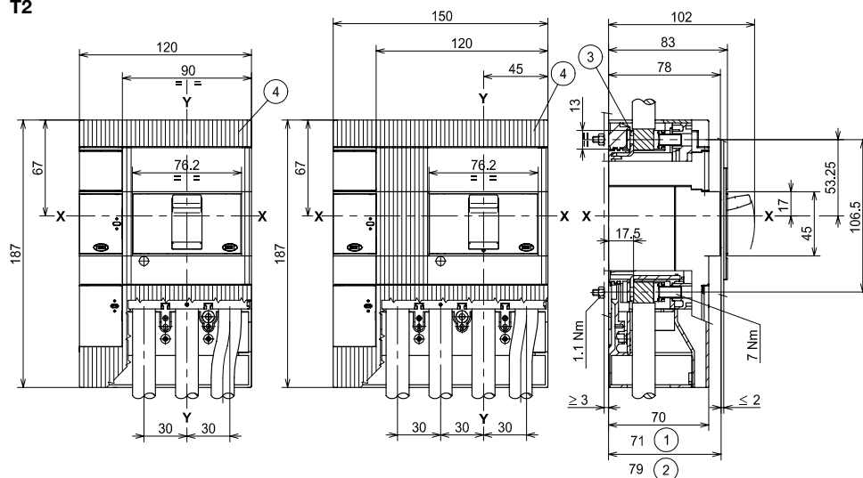
T2
