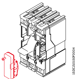
AUX-C
