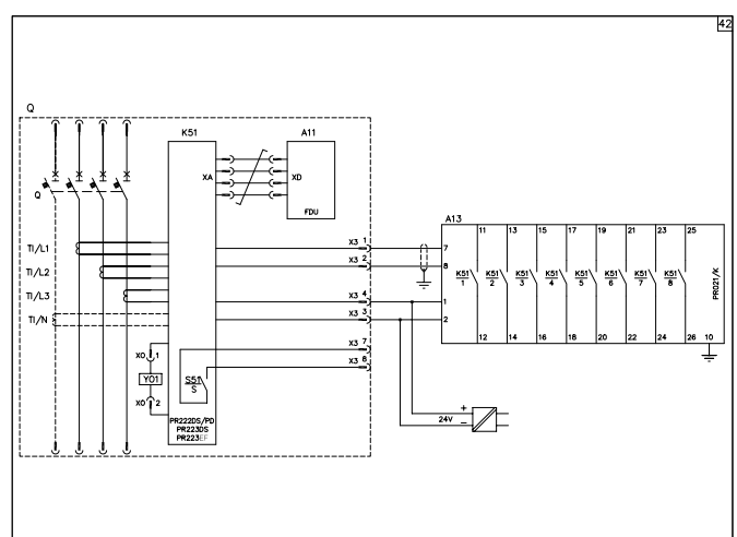
PR222DS/PD和PR223DS或PR223EF电子脱扣器与PR021/K信号单元的连接
