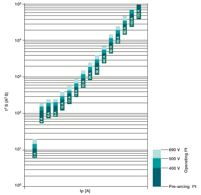
Characteristic I^2t
