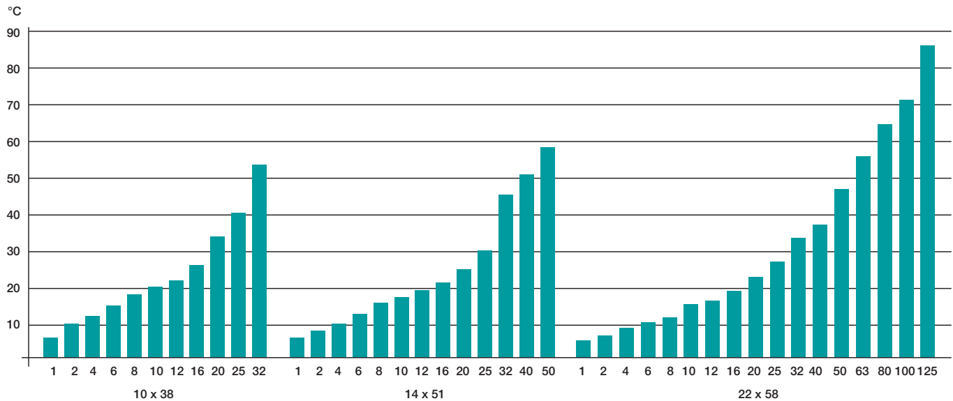
Temperature increase
