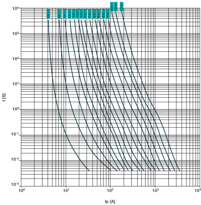
Characteristic tI
