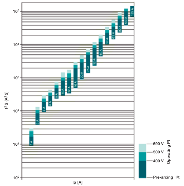
Characteristic I^2t
