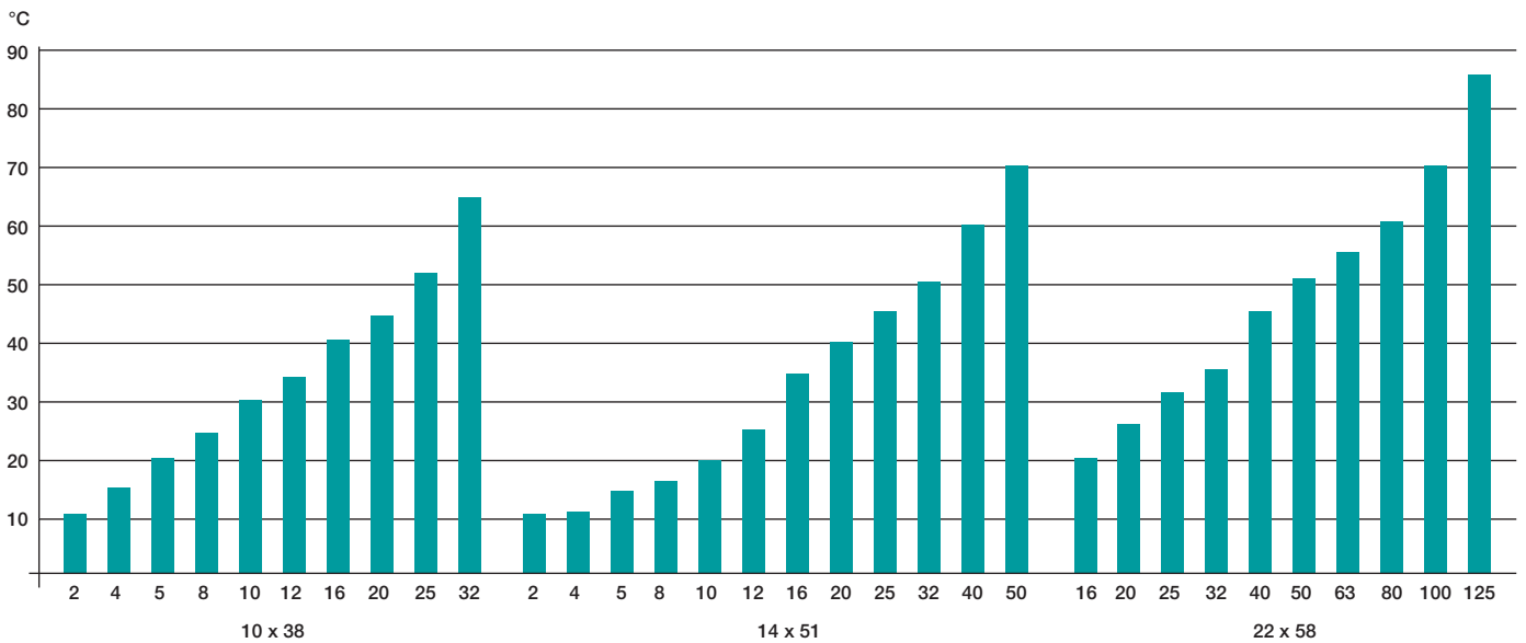
Temperature increase
