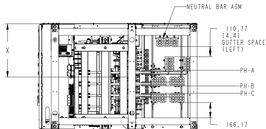
TOP VIEW PANEL REMOVED (3 POLE UNIT)
