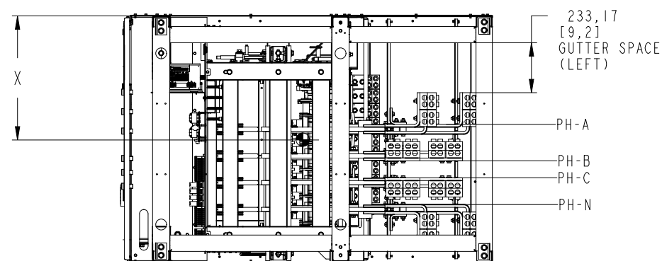
TOP VIEW PANEL REMOVED (4 POLE UNIT)
