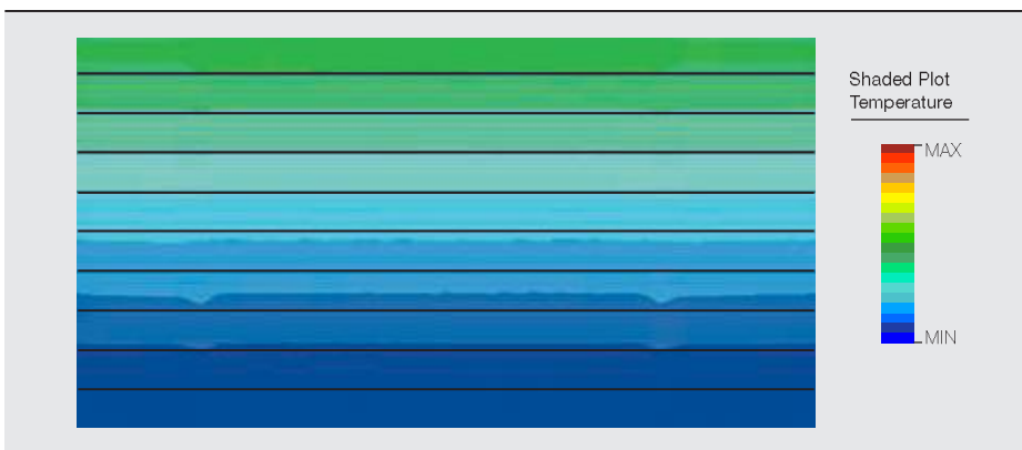
4 Temperature distribution for tank LV wall for the original model of investigated transformer
