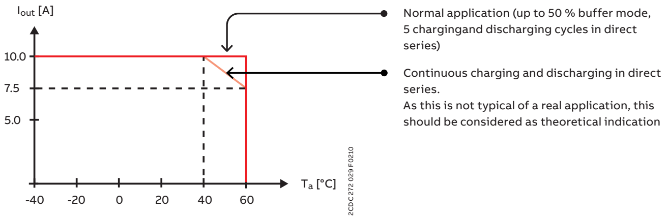
Characteristic curve of the temperature at rated load
