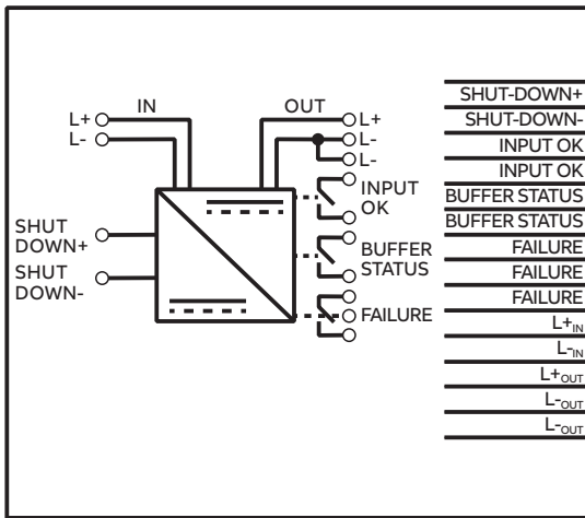
Connection diagram
