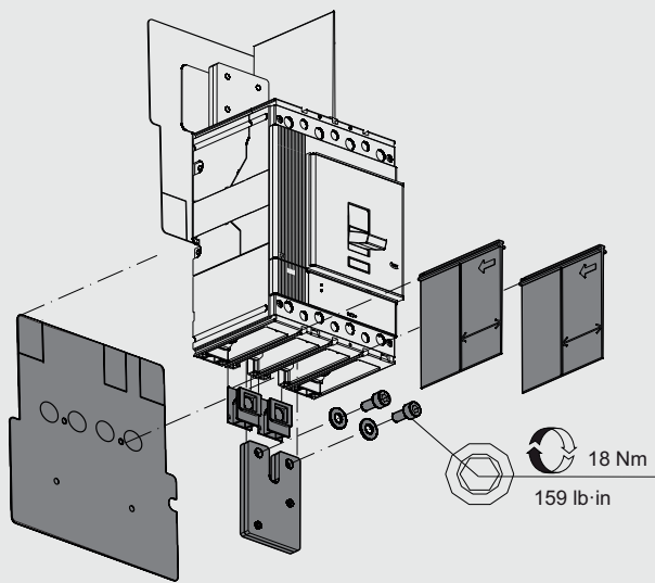
I 2PS+2PS solution, Lower Supply
