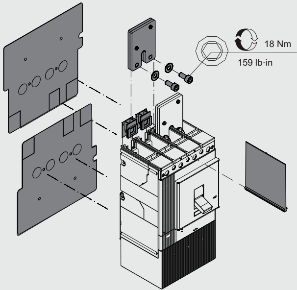
Example for 2P+2PS (Lower Supply)
