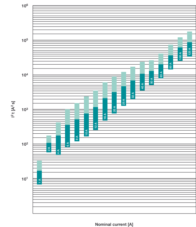
Characteristic I²t
