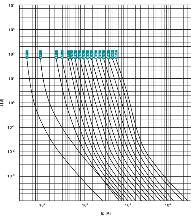
Characteristic tI
