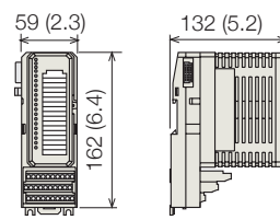
Compact I/O
