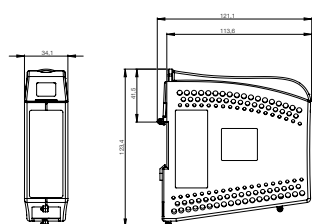
NE801/802
