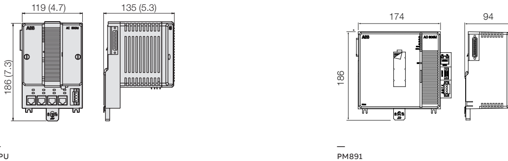
CPU
