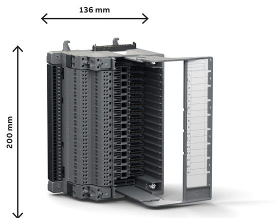
TUS810 Select I/O MTU
