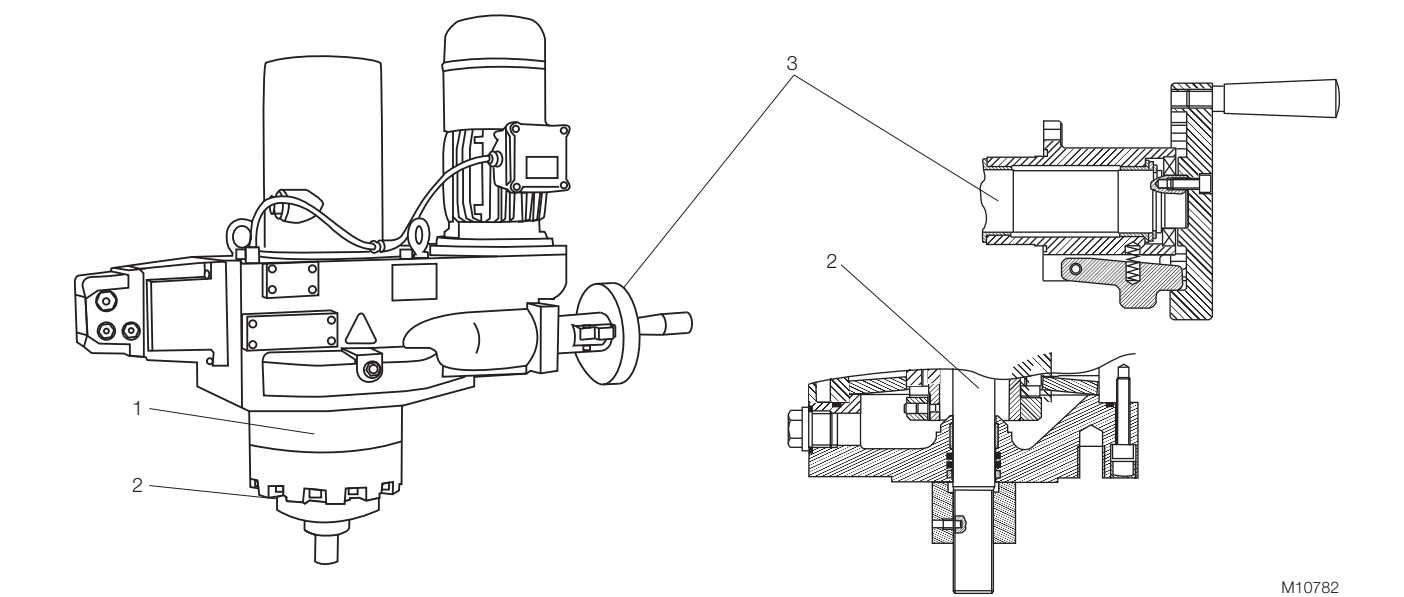
Fig. 8: Gasket sets and handwheel drive
