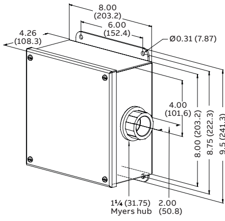
80 kA metal enclosure pre-wired Enclosure option M
