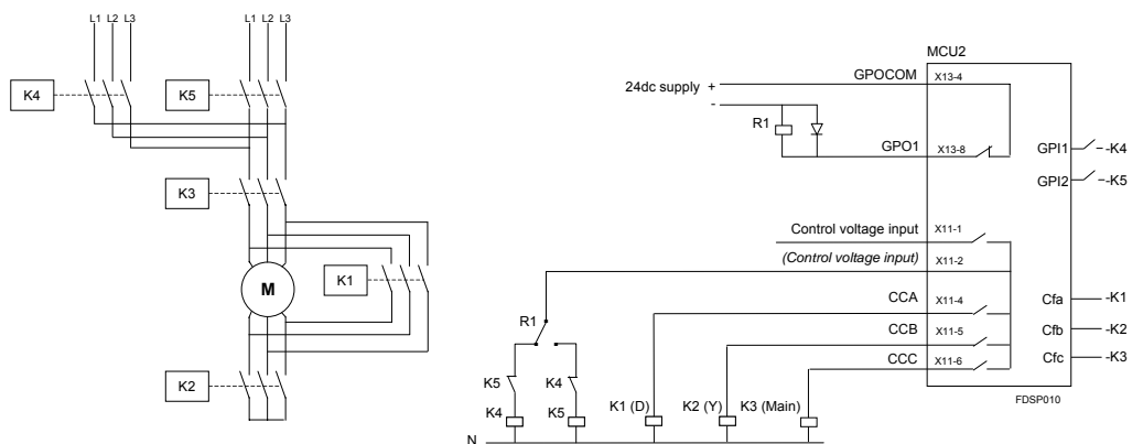
Picture 24. Control circuit for REV-S/D starter, MCU2.
