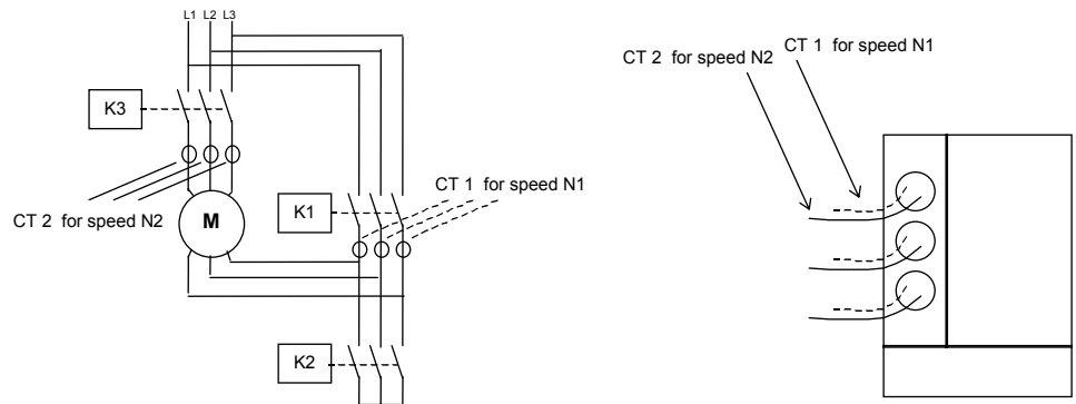
Picture 27. External current transformer connection for NR-2N to MCU2 unit.
