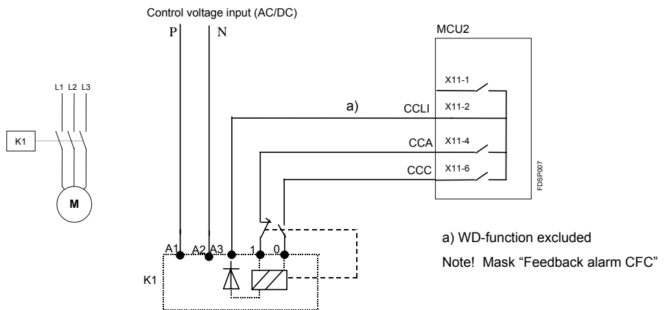
Picture 12. Control circuit for latched NR-DOL, magnetic latched contactor.
