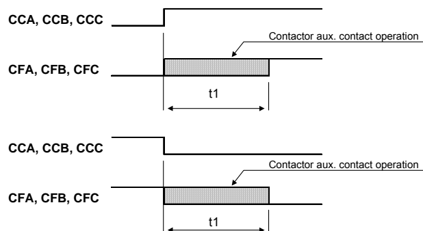
Picture 55. Contactor operation within Feedback delay .
