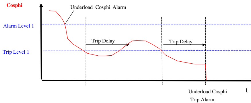
Picture 45. Underload cosphi protection.
