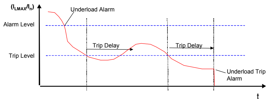
Picture 44. MCU underload protection.
