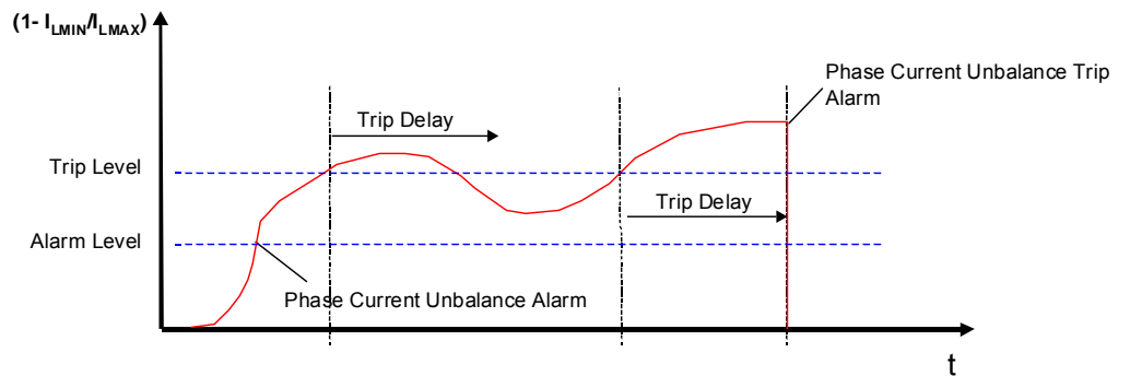
Picture 49. MCU2 unbalance protection.
