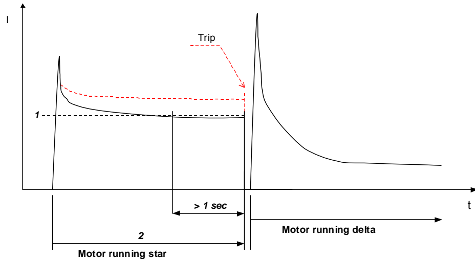
Picture 23. NR-S/D switching over parameters, principle picture.
