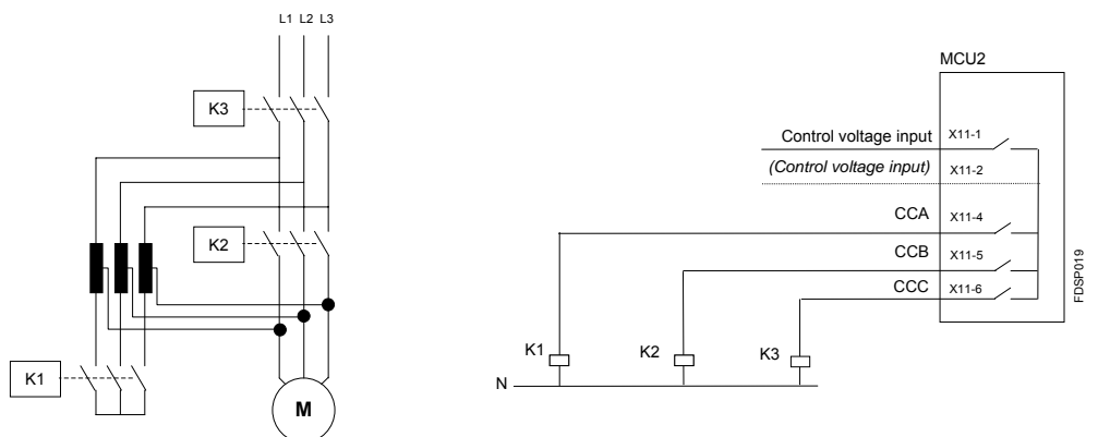
Picture 34. Control circuit for autotransformer starter, example 3.
