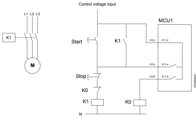
Picture 19. Control circuit for NR-DOL/RCU starter for MCU1.
