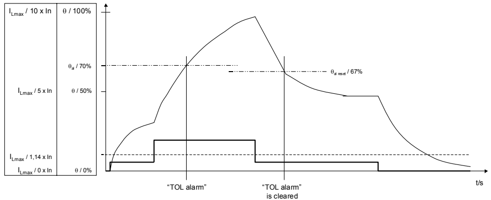
Picture 38. TOL alarm indication ( TOL alarm level , \theta_{al} and alarm reset, \theta_{al\ reset} ).
