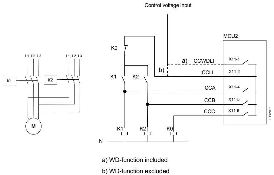
Picture 11. Control circuit for latched NR-DOL, mechanical latched contactor.
