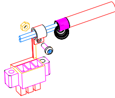
Picture 6. Fieldbus cable shield and fieldbus connector.
