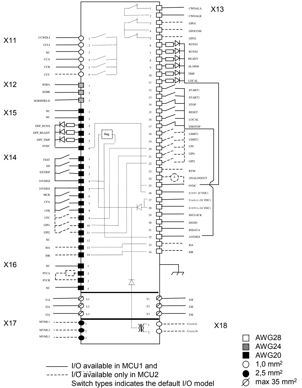
Picture 57. Terminals for MCU1-4 and MCU2-4.
