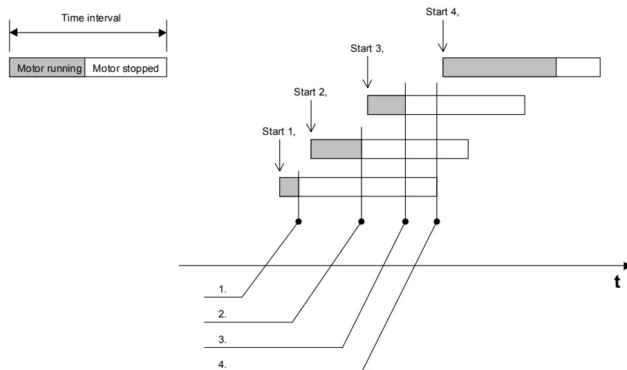
Picture 53. Start limitation for Number of starts 3 within Time interval .
