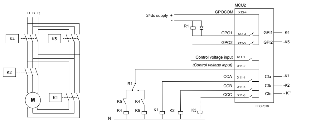
Picture 29. Control circuit for REV-2N starter with separate windings.
