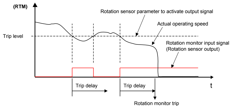
Picture 50. MCU2 rotation monitor protection.
