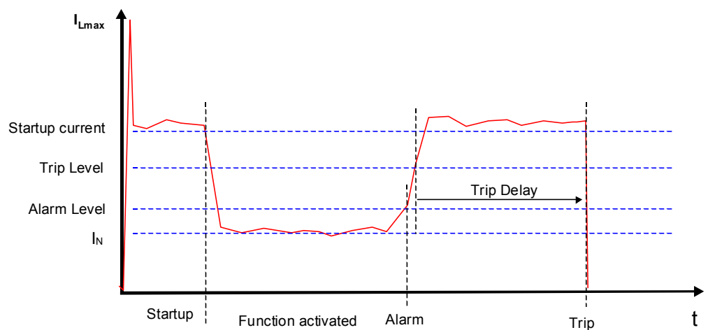
Picture 47. MCU stall protection.
