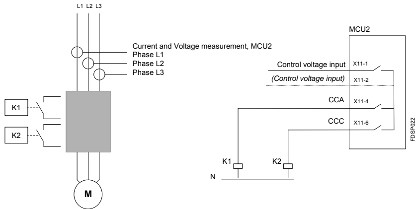
Picture 15. Control circuit with softstarter for NR-DOL, latched contactors.
