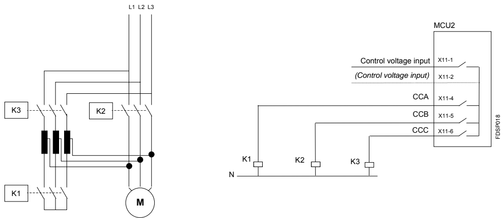
Picture 32. Control circuit for autotransformer starter, example 1, MCU2.
