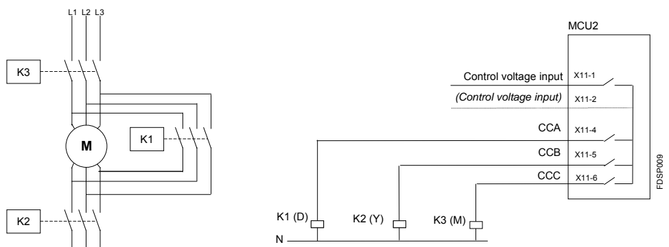
Picture 22. Control circuit for NR-S/D starter, MCU2.
