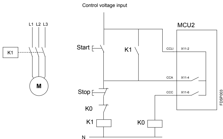
Picture 20. Control circuit for NR-DOL/RCU starter for MCU2.
