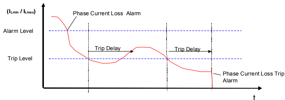
Picture 43. MCU phase current loss protection.
