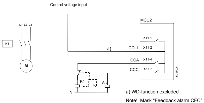
Picture 12. Control circuit for latched NR-DOL, magnetic latched contactor.
