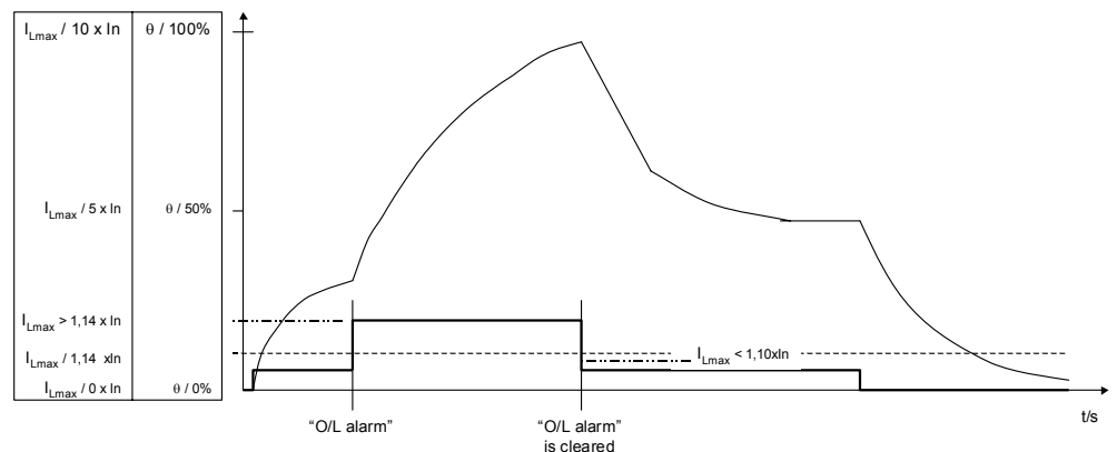
Picture 39. Thermal protection overload alarm indication.
