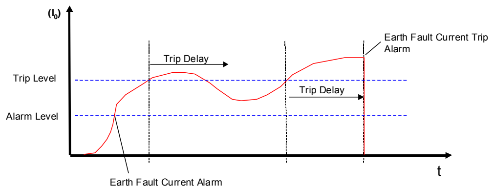
Picture 48. MCU2 earth fault protection.
