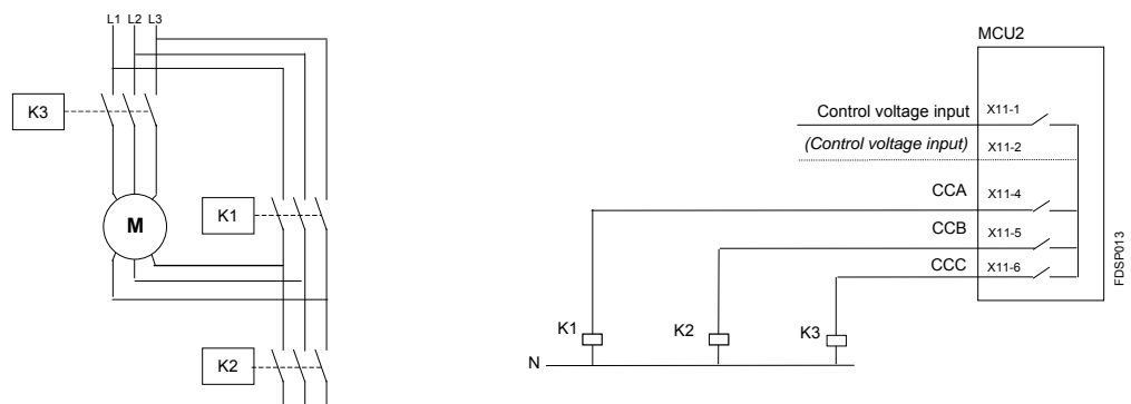
Picture 25. Control circuit for NR-2N starter, Dahlander, MCU2.
