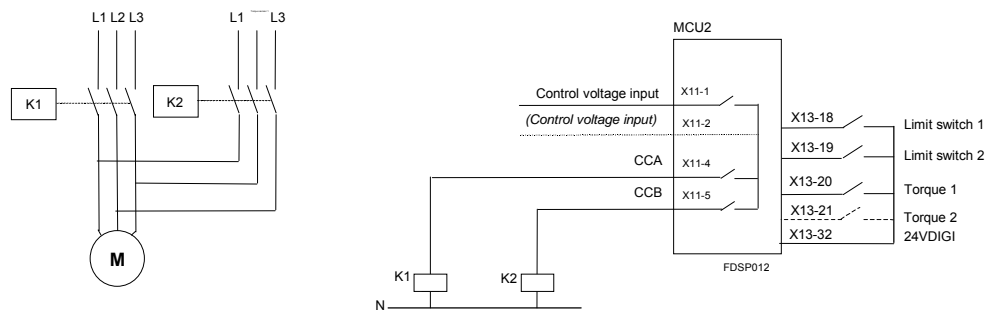
Picture 31. Control circuit for Actuator starter with torque switch, MCU2.
