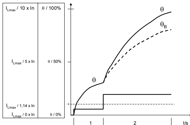
Picture 40. Thermal level increase during motor operating condition.
