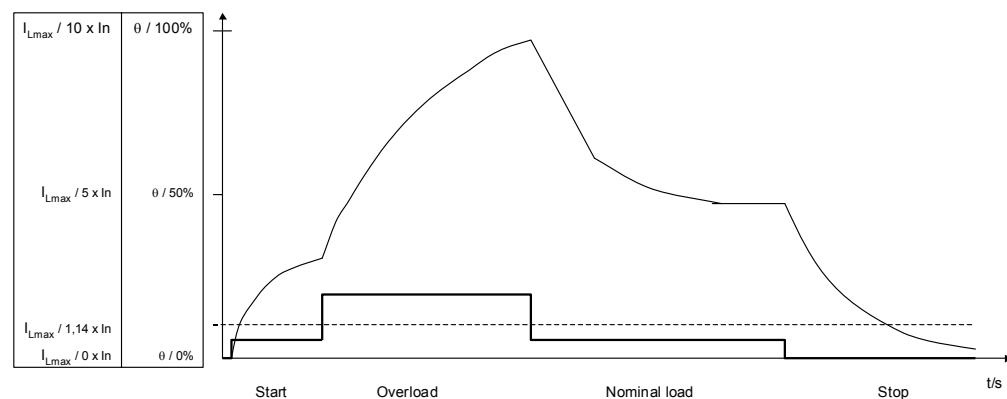
Picture 35. Principle picture of motor thermal simulation.
