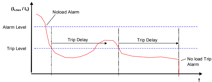
Picture 46. MCU no load protection.
