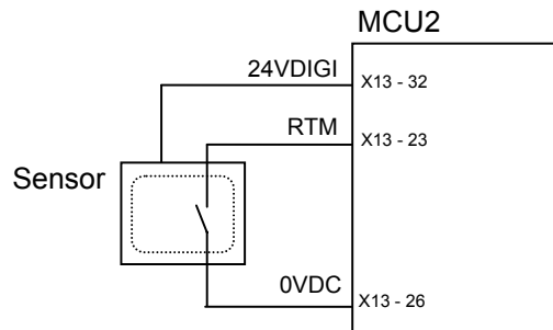
Picture 5. Connection of the rotation monitor sensor.
