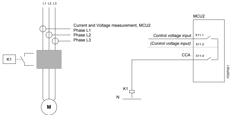
Picture 13. Control circuit with softstarter for NR-DOL, MCU2.
