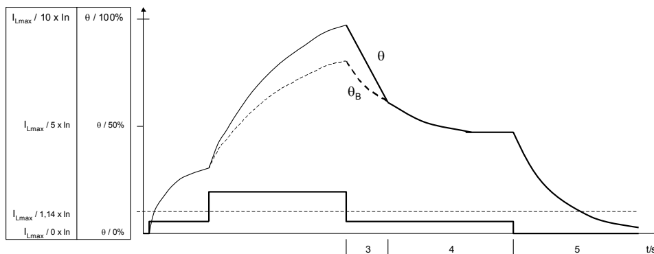
Picture 41. Cooling down for a stopped or running motor.
