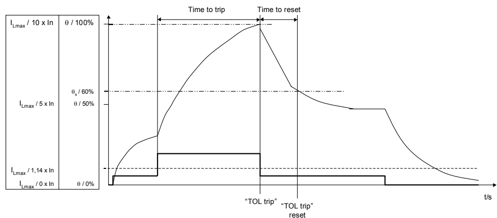
Picture 37. Thermal protection trip functionality (trip reset level, \theta_s ).
