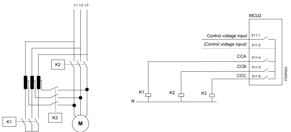
Picture 34. Control circuit for autotransformer starter, example 3.
