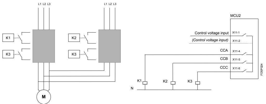
Picture 16. Control circuit with softstarter for REV-DOL, latched contactors.
