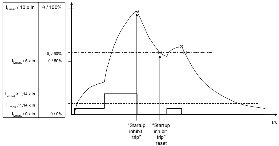
Picture 36. Startup inhibit level functionality.
