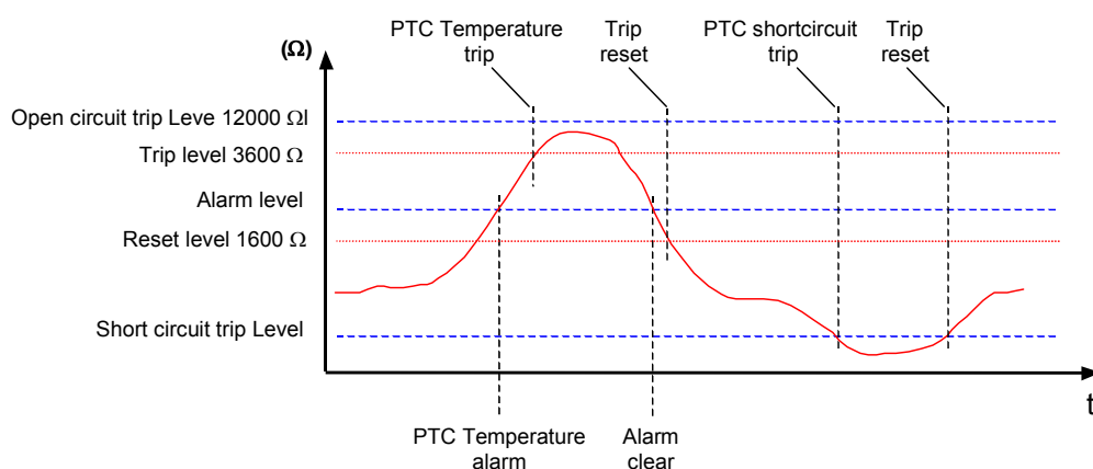
Picture 51. Thermal protection with PTC.
