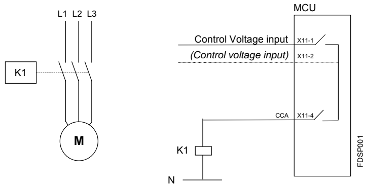
Picture 7. Contactor control wiring for NR-DOL starter, MCU1 and MCU2.
