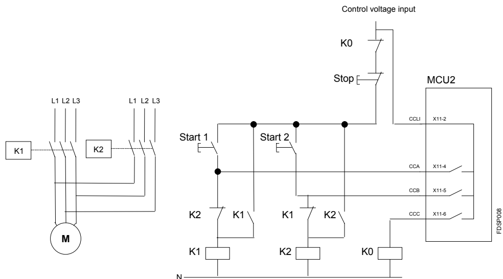
Picture 21. Control circuit for REV-DOL/RCU starter, MCU2.
