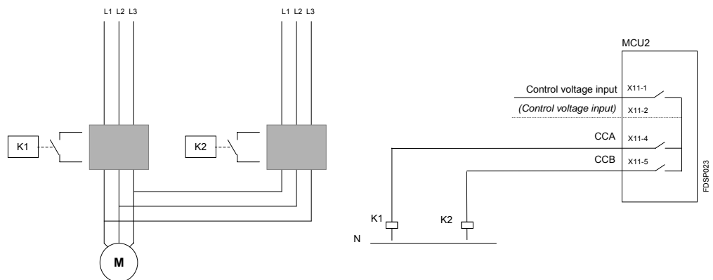
Picture 14. Control circuit with softstarter for REV-DOL, MCU2.
