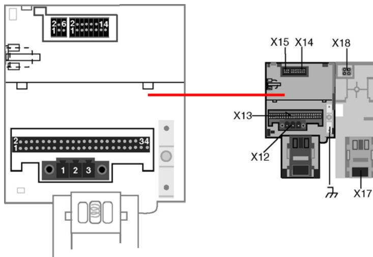
Picture 4. Connectors on the side of the unit.
