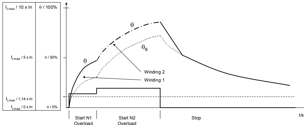
Picture 42. Thermal simulation principle for two speed motor.
