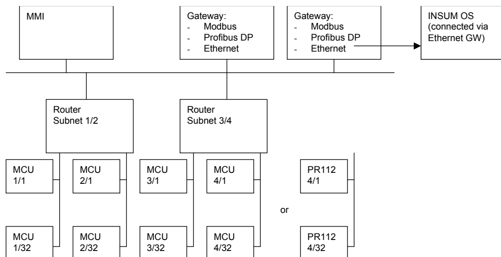
Picture 2. INSUM system configuration with Motor Control Units (MCU).
