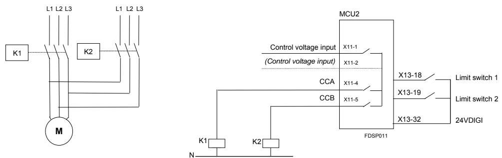
Picture 30. Control circuit for Actuator starter with limit switches, MCU2.
