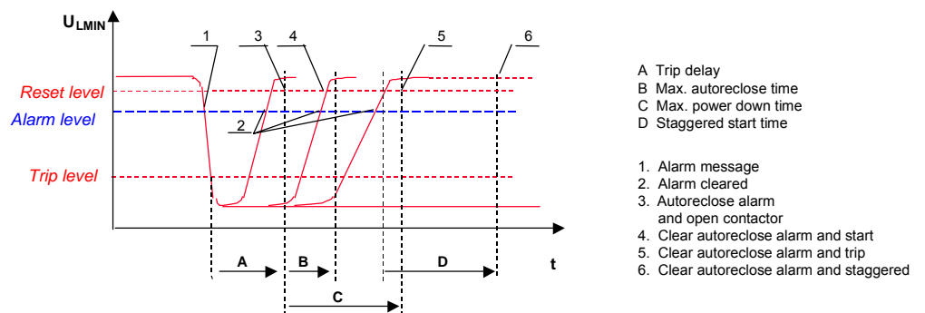
Picture 52. Undervoltage protection function.
