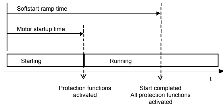
Picture 17. Start sequences for softstarter with delay times.
