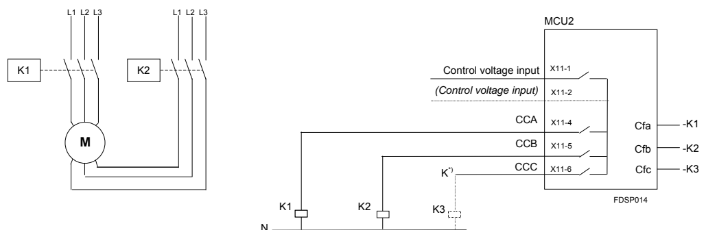
Picture 26. Control circuit for NR-2N with two contactors, separate windings, MCU2.
