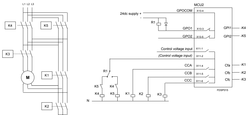
Picture 28. Control circuit for REV-2N starter, reversing Dahlander.
