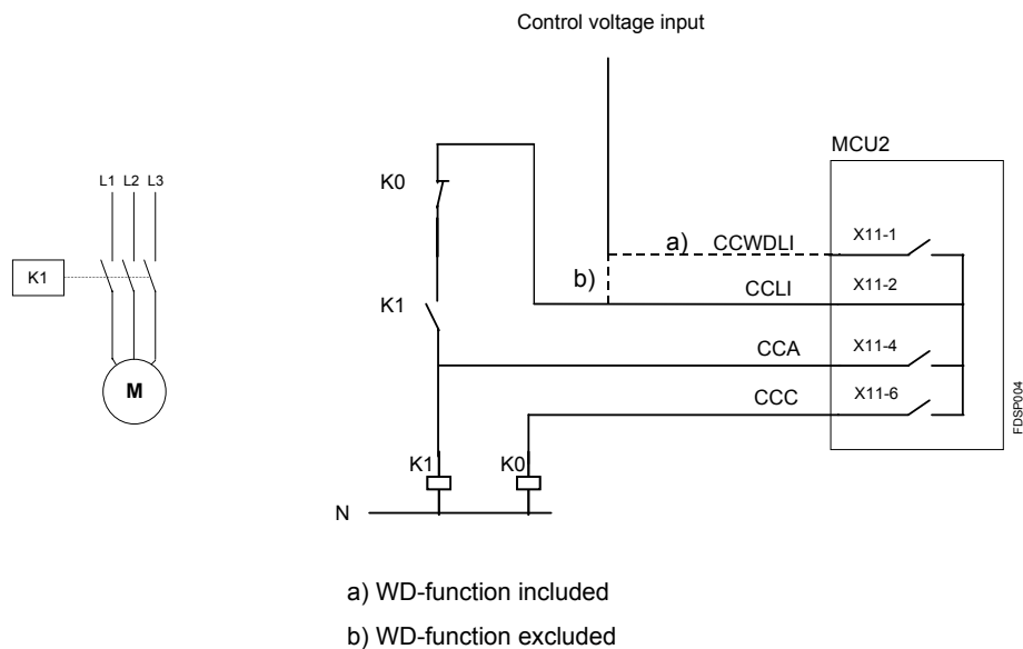
Picture 9. Control circuit for latched NR-DOL with normal contactors, MCU2.
