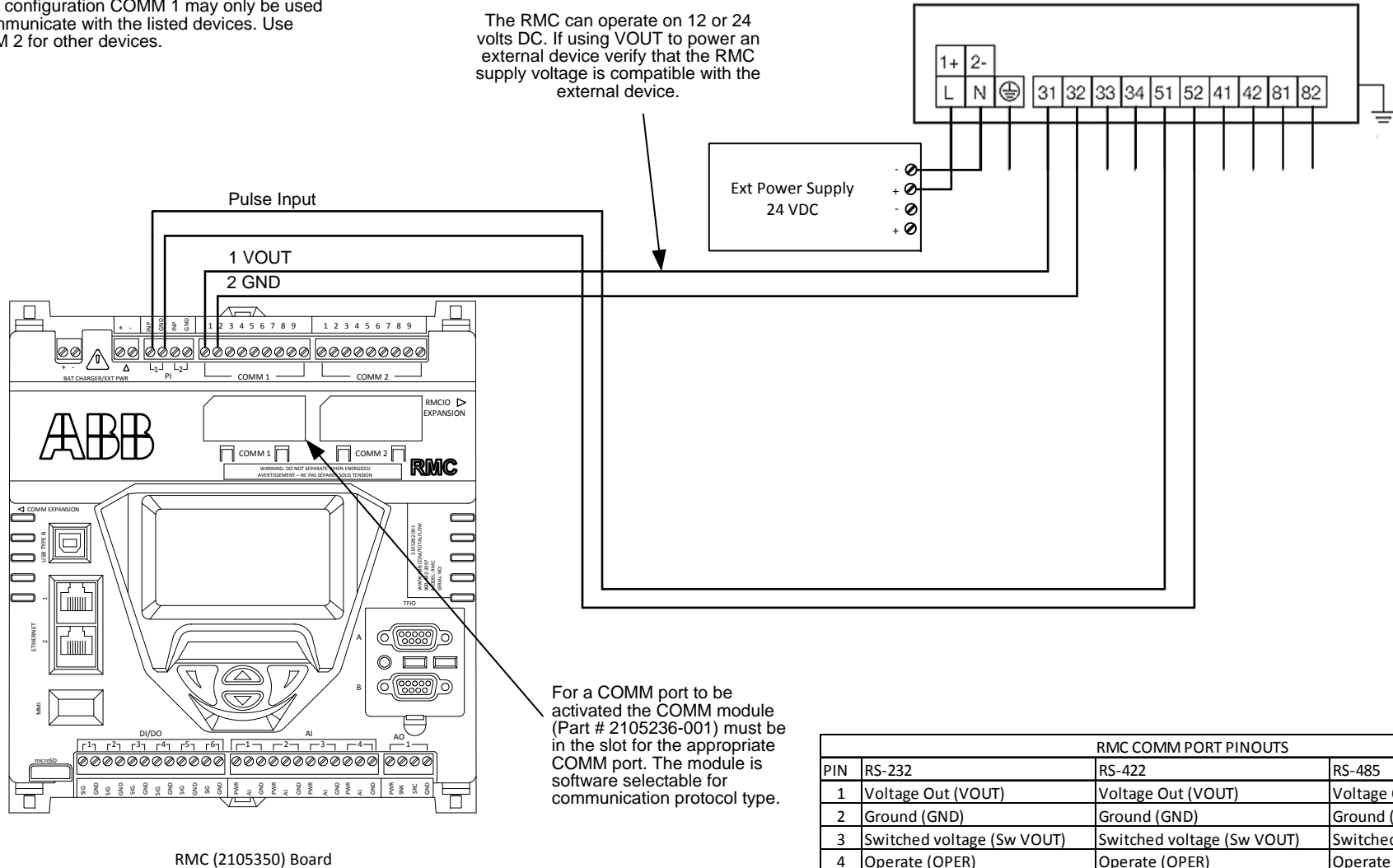
RMC (2105350) Board
