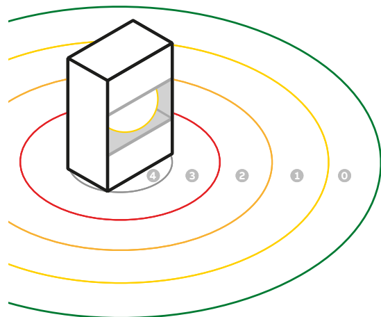
Fig. 12. Arc flash boundary energy zones
