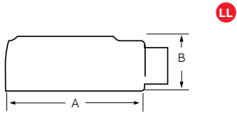
LL Form 7 ferrous conduit bodies with covers
