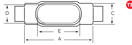
TB Mark 9 aluminum conduit bodies with covers
