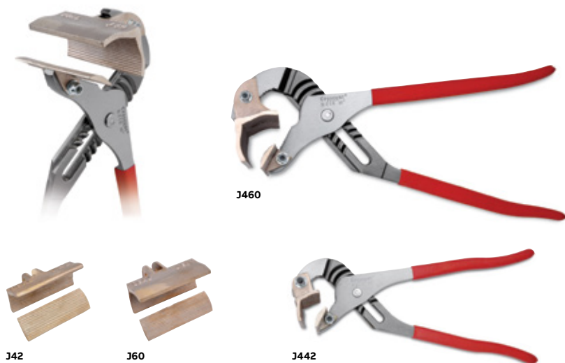
Ocal J-wrenches
