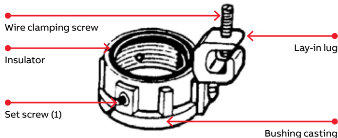
3870 Series
