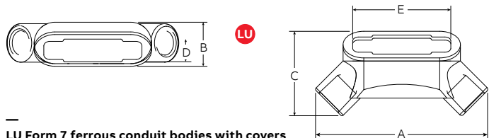
LU Form 7 ferrous conduit bodies with covers
