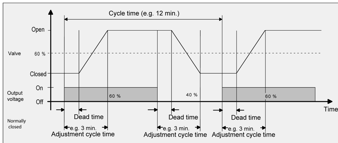
Figure 41: Ideal course of the valve stroke for a command value of approx. 60 % of a deenergised, closed valve
