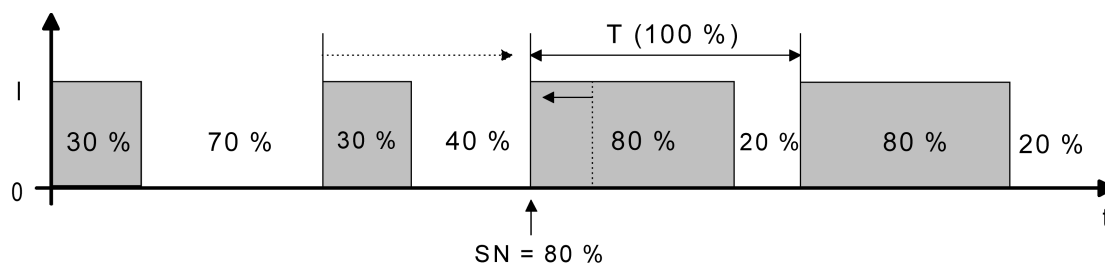
Figure 40: Command value change, e.g. from 30 % to 80 % during the closing phase of the valve (closing phase too long)
