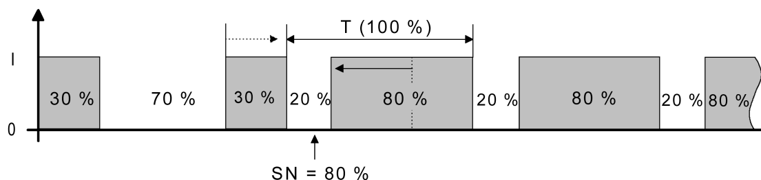
Figure 39: Command value change, e.g. from 30 % to 80 % during the closing phase of the valve
