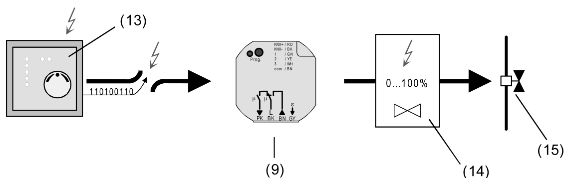
Figure 43: Principle of cyclical command value monitoring in the event of a fault (e.g. open circuit)
