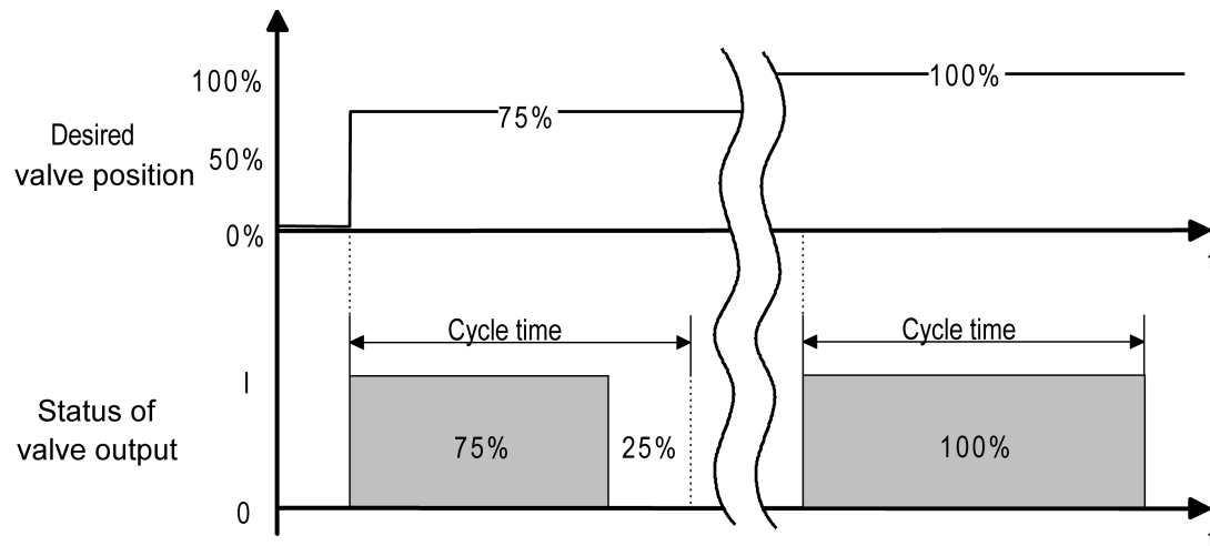
Figure 29: Conversion of a constant valve setpoint position to an output signal with deenergised, closed valve drives (example)
