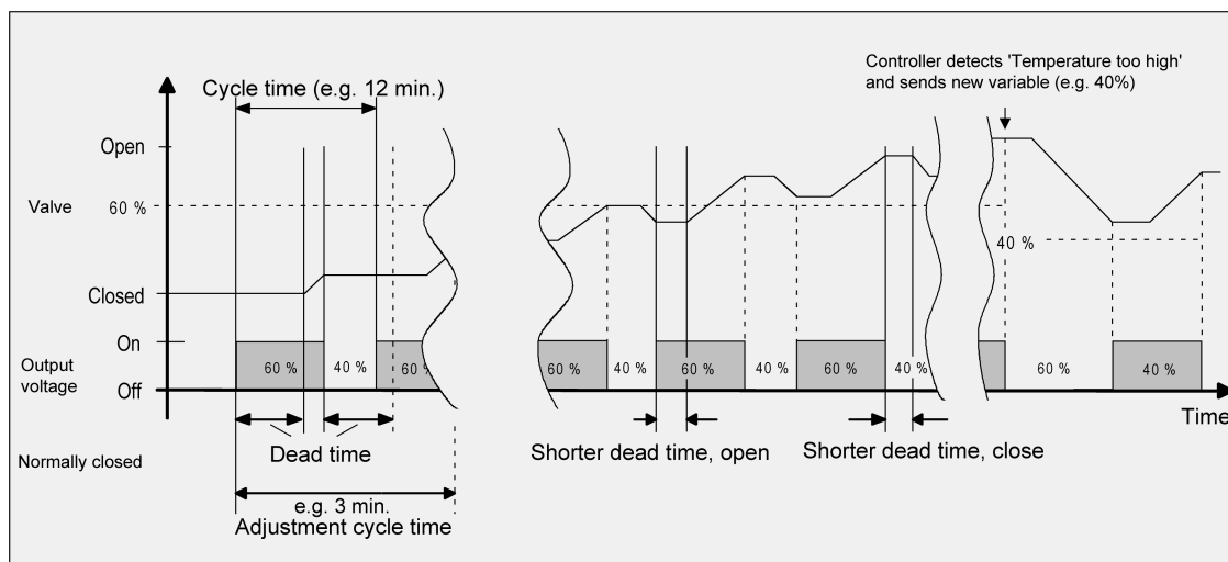
Figure 42: Ideal course of the valve stroke for a command value of approx. 60 % at first of a deenergised, closed valve
