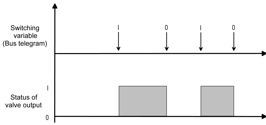
Figure 28: Conversion of a switching command value to an output signal with deenergised, closed valve drives (example)
