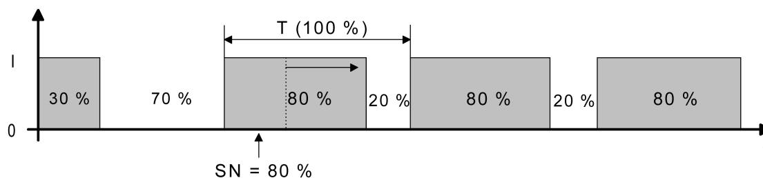
Figure 38: Command value change, e.g. from 30 % to 80 % during the opening phase of the valve
