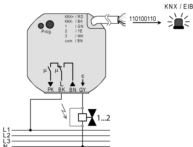
Figure 44: Short-circuit and overload detection in case of fault in valve output or valve drive
