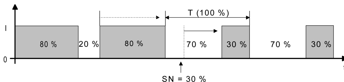
Figure 36: Command value change, e.g. from 80 % to 30 % during the closing phase of the valve
