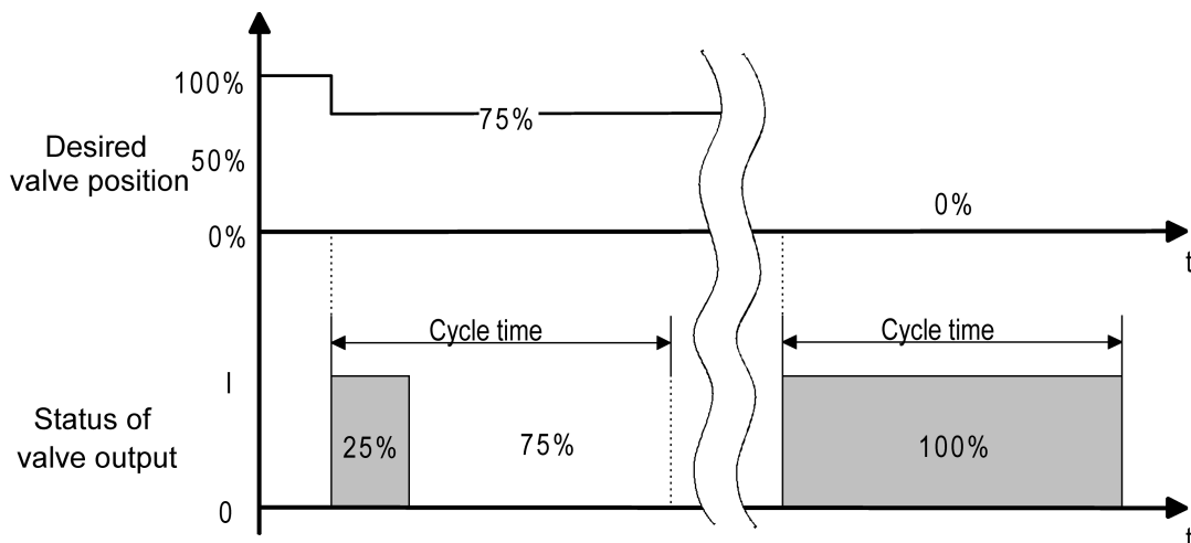
Figure 31: Conversion of a constant valve setpoint position to an output signal with deenergised, opened valve drives (example)
