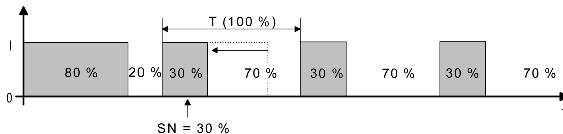
Figure 35: Command value change, e.g. from 80 % to 30 % during the opening phase of the valve
