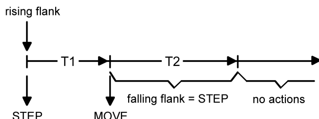
Figure 7: Operation concept "short – long – short"
