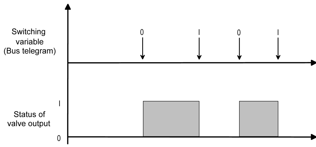
Figure 30: Conversion of a switching command value to an output signal with deenergised, opened valve drives (example)
