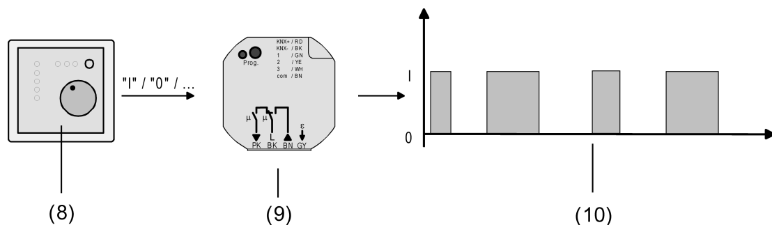
Figure 32: Command value principle for switching command value
