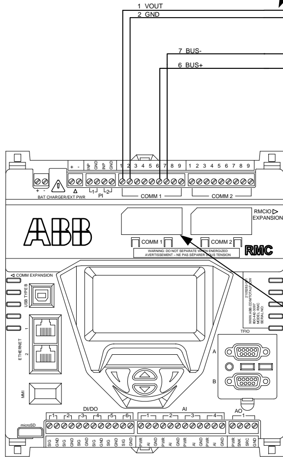
RMC (2105350) Board
