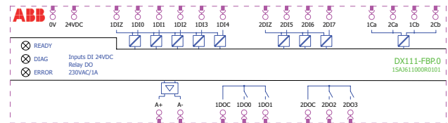
Example for a DX111 ePLAN macro variant B
