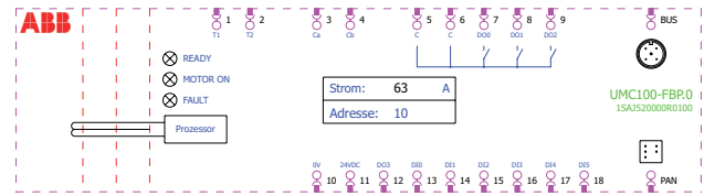
Example for a UMC100 ePLAN macro variant A
