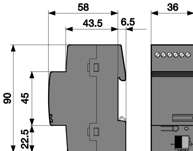
Fig. 8: Dimensiones BI-M-4.0.1
