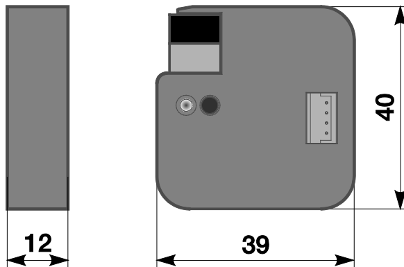
Fig. 6: Dimensiones BI-F-2.0.1
