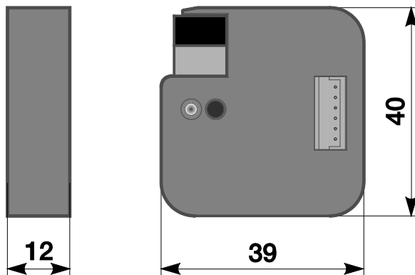
Fig. 7: Dimensiones BI-F-4.0.1
