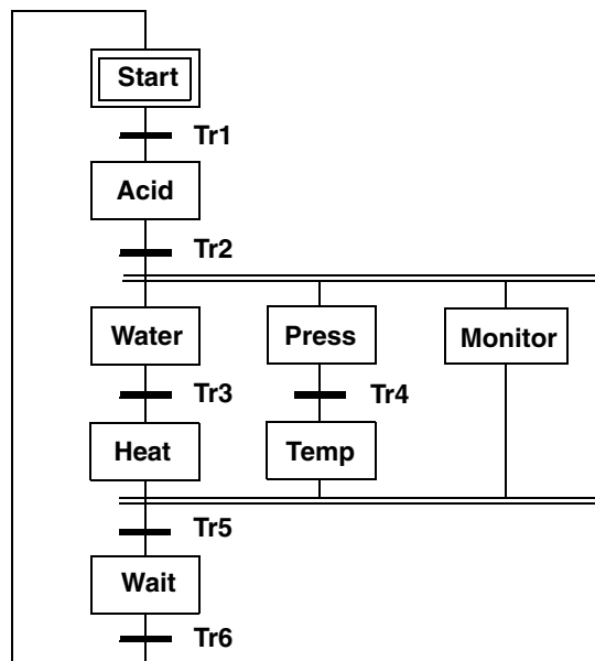
Figure 36. Example of a simultaneous sequence with three continuous branches
