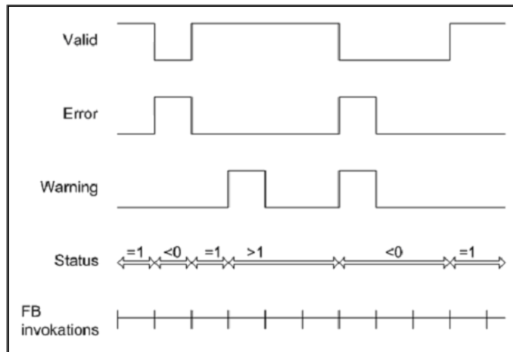
Figure 39. Enable always true
