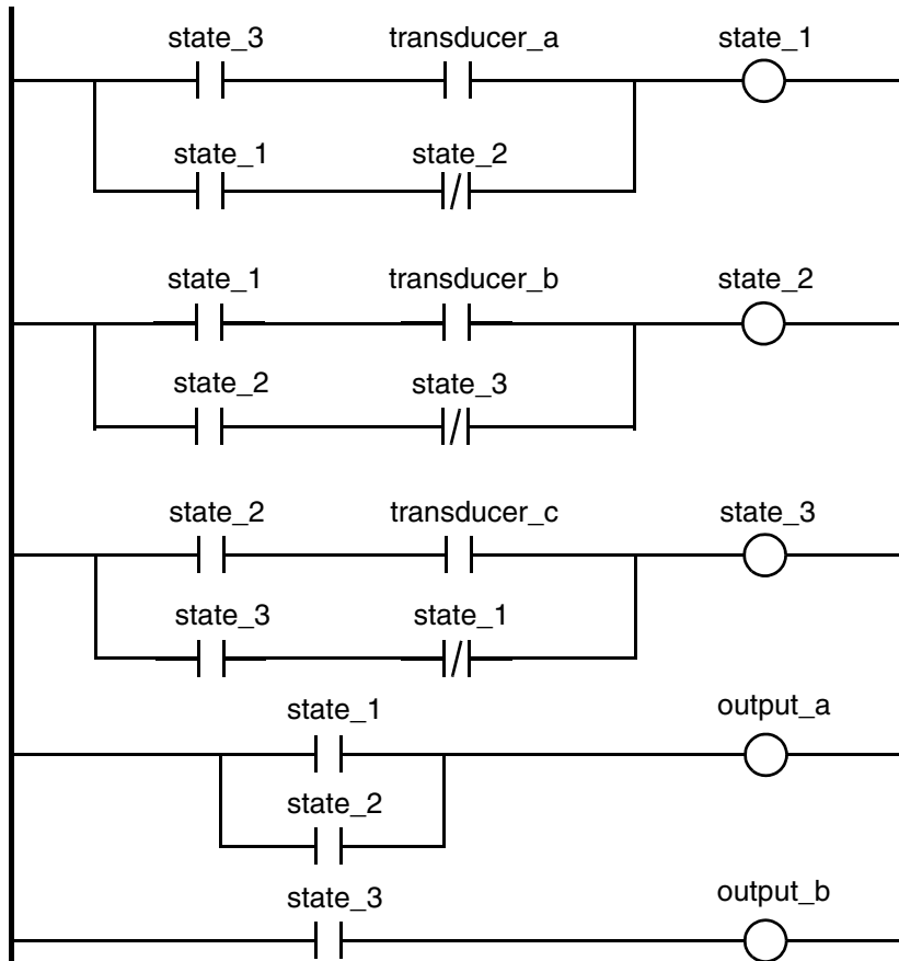
Figure 29. Sequence program with three states controlling two outputs
