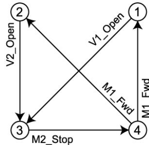
Figure 56. Analyze of the Code Block 3 dependency
