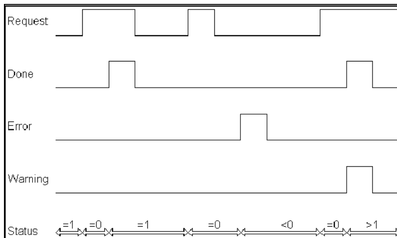
Figure 42. Examples of event-driven execution
