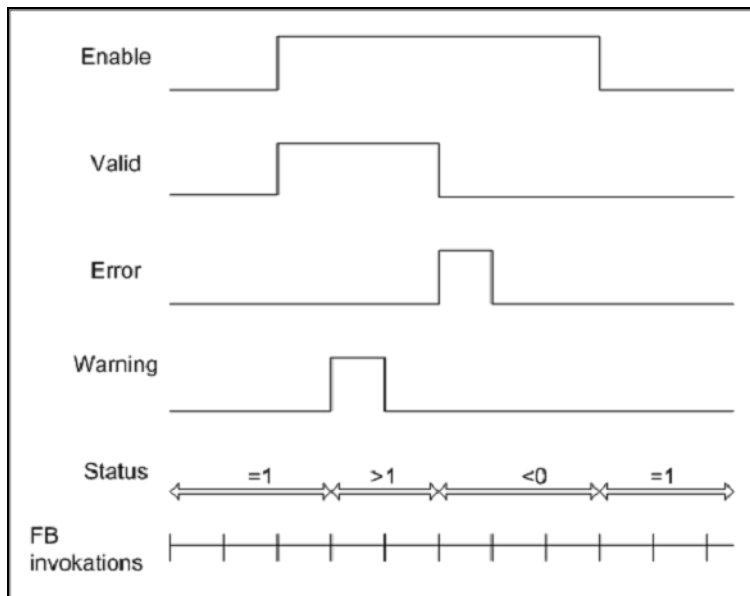
Figure 40. Direct response on activation/deactivation
