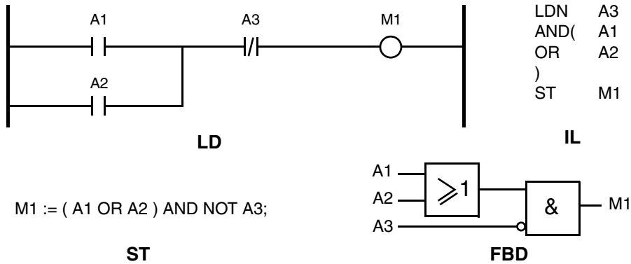
Figure 16. A Boolean condition programmed with four of the five IEC 61131-3 programming languages. SFC is normally only used for sequences
