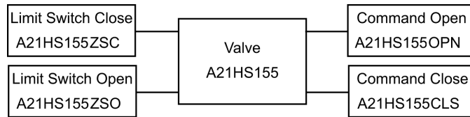
Figure 62. Digital or Boolean control
