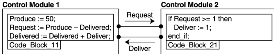
Figure 49. Control module 2 reads Request and writes Deliver, and control module 1 reads Deliver and writes Request. This execution order cannot be resolved
