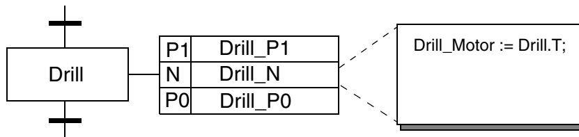
Figure 34. Example of a step with the associated actions folded out and one of them described in a separate editor window
