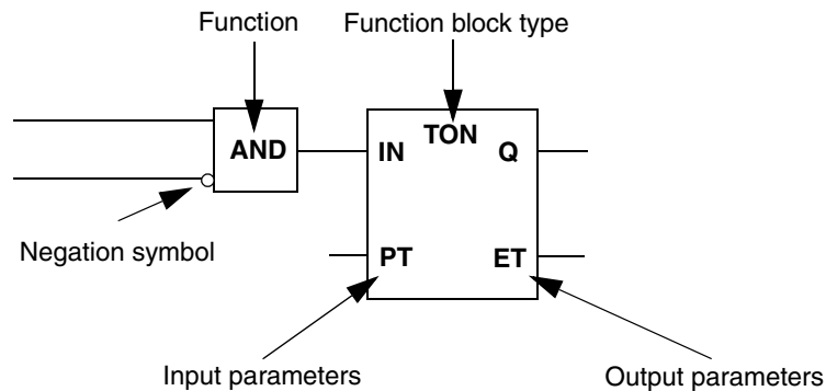
Figure 19. Some fundamental rules for drawing function block diagrams
