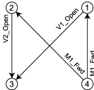
Figure 55. Analyze of the Code Block 2 dependency
