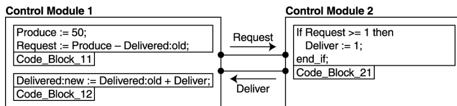
Figure 51. How to eliminate code loop dependencies
