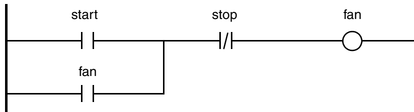
Figure 27. Feedback loop in an LD program. The fan starts with an impulse on contact start and continues to run until the contact stop is opened
