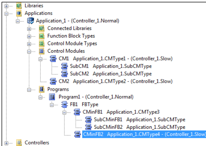
Figure 38. Example of task connection to a sub control module
