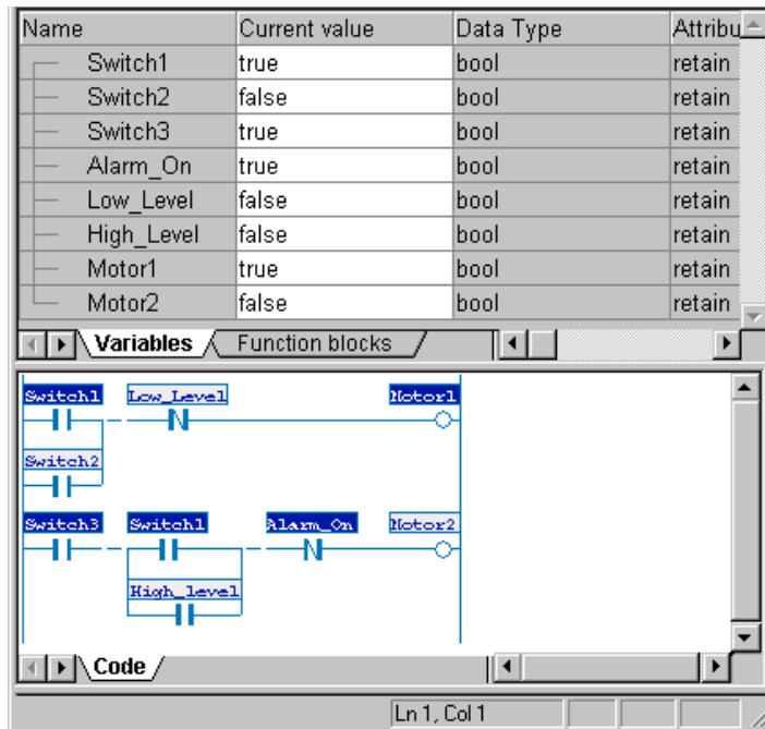
Figure 28. Status indication of an executing LD program
