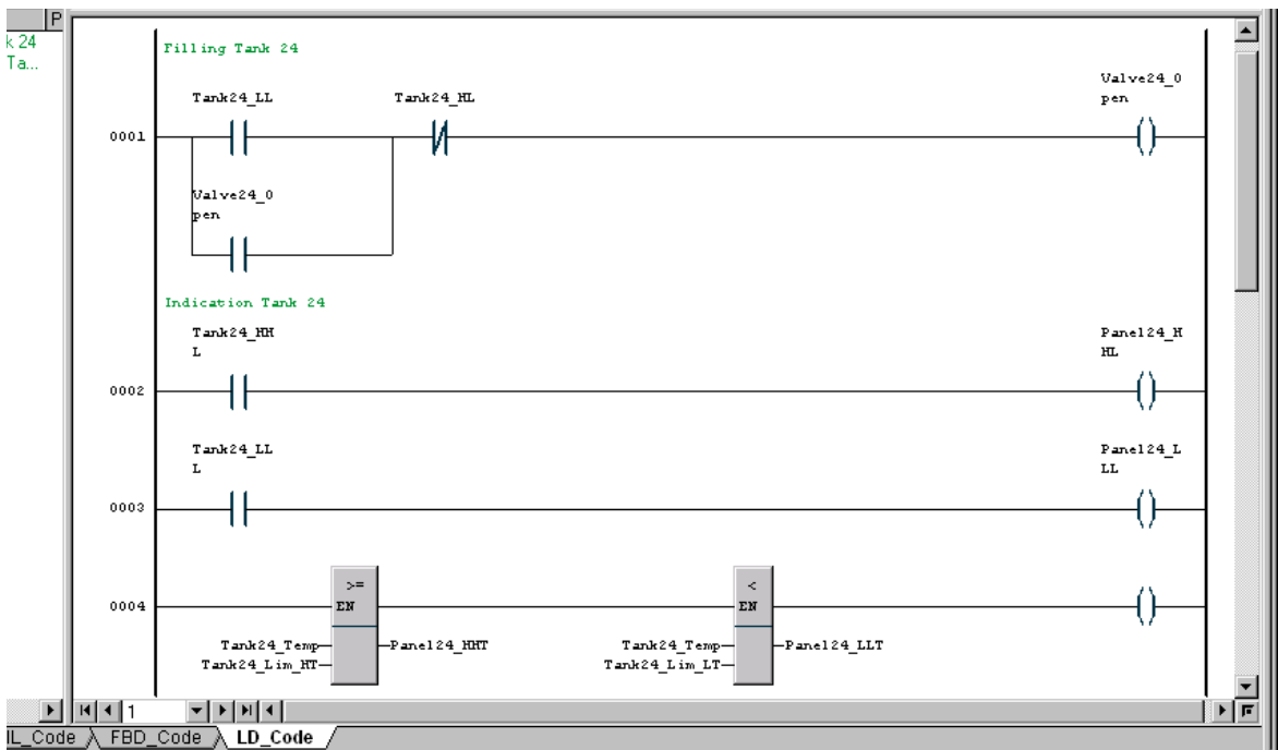
Figure 26. Example of LD code
