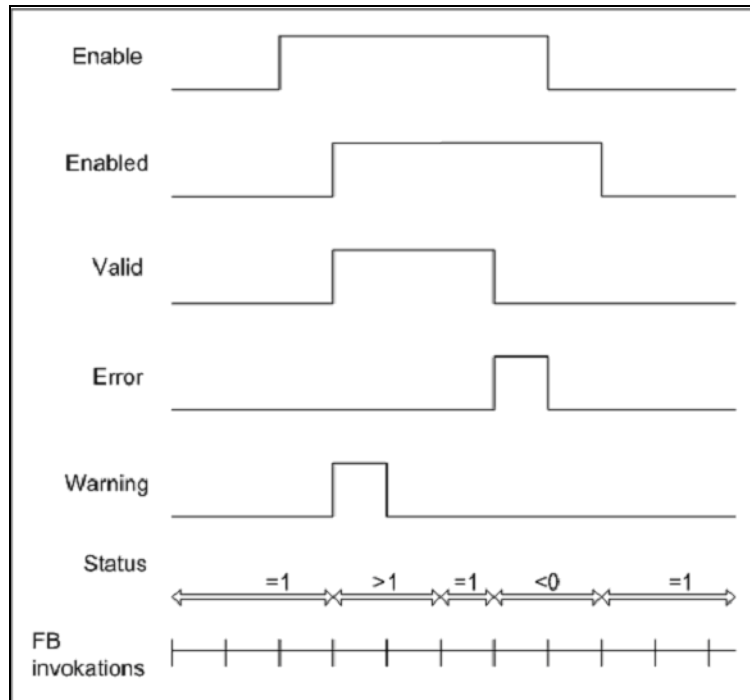
Figure 41. Delayed response on activation/deactivation
