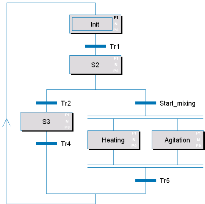
Figure 31. Example of a sequence structure. In the box Init P1 contains code, N and P0 are empty
