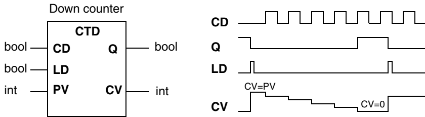
Figure 24. Example of a CTD counter block with preset value PV=5
