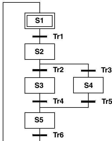
Figure 35. Example of a sequence selection with two branches
