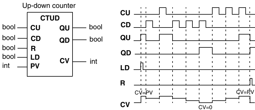
Figure 25. Example of a CTUD counter block with preset value PV=3
