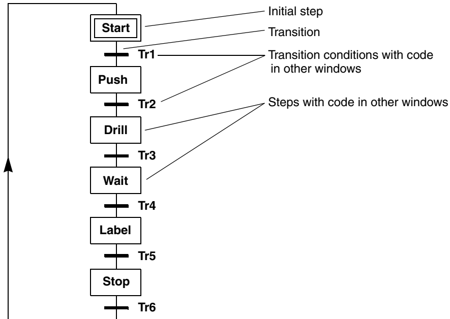
Figure 33. Example of an SFC program for an automatic drilling machine. Note the cyclic execution being enabled by the Tr6 transition condition
