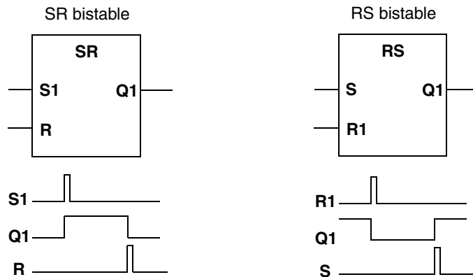
Figure 20. SR and RS bistable symbols with their corresponding functions below
