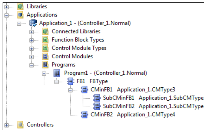
Figure 37. Control modules in function blocks example
