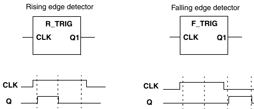
Figure 21. Edge detectors create a single pulse with the same duration as the execution time of the function block
