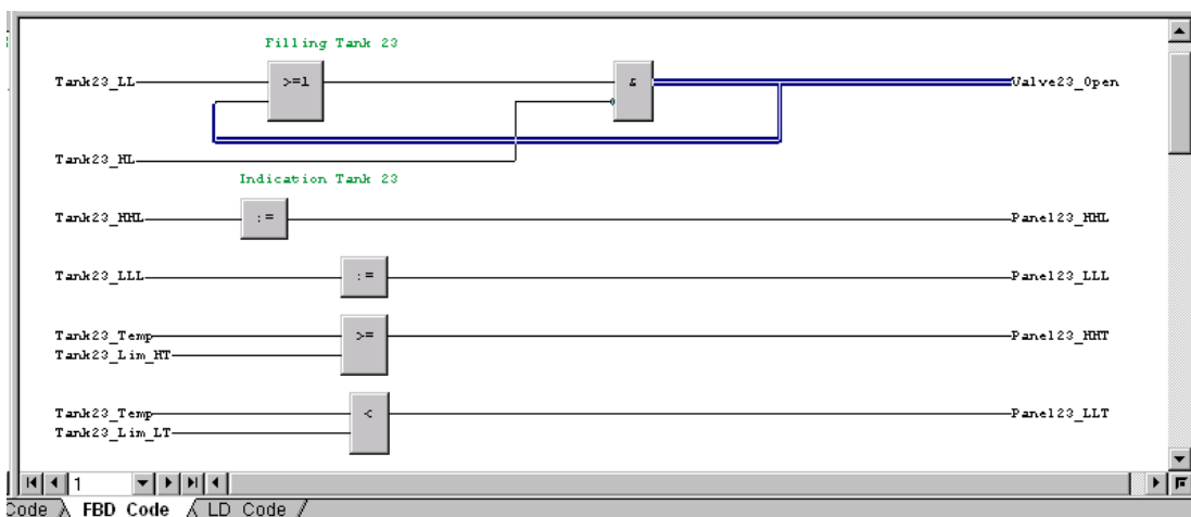
Figure 18. Example of FBD code
