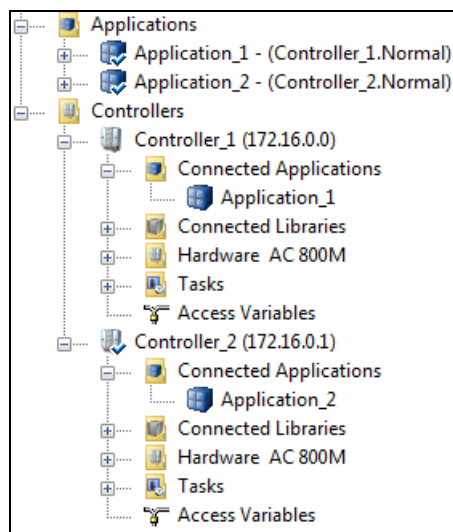
Figure 13. Project Explorer configuration with two controllers, each with one application
