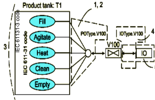
Figure 43. Using structured Data Types to communicate between IO and the application
