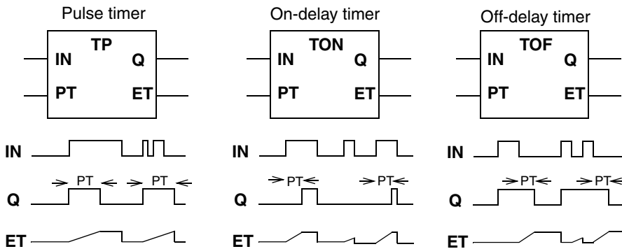
Figure 22. Timing diagrams for the three different types of timer function blocks
