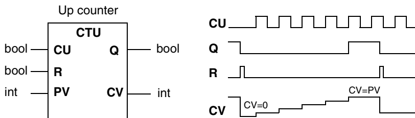
Figure 23. Example of a CTU counter block with preset value PV=5
