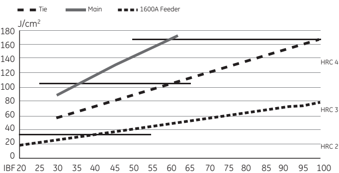
Figure 4.5 Arc Flash Energy, Main Bus and Feeder with Selective Delays
