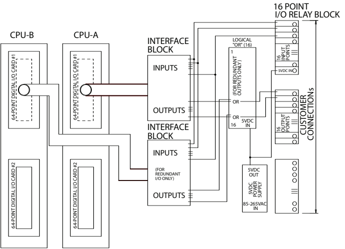
Figure 10.1 Redundant Digital I/O Hardware Configuration
