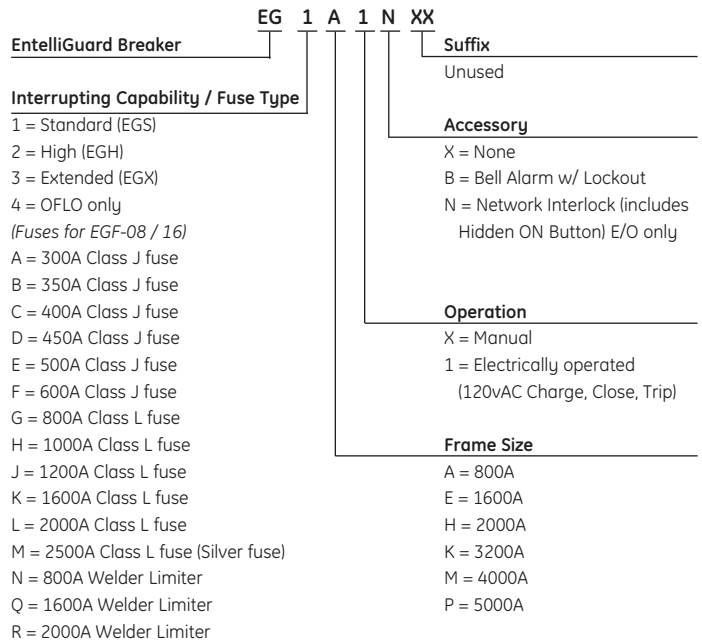
Figure 5.2 EntelliGuard Low-Voltage Power Circuit Breaker Catalog Numbers
