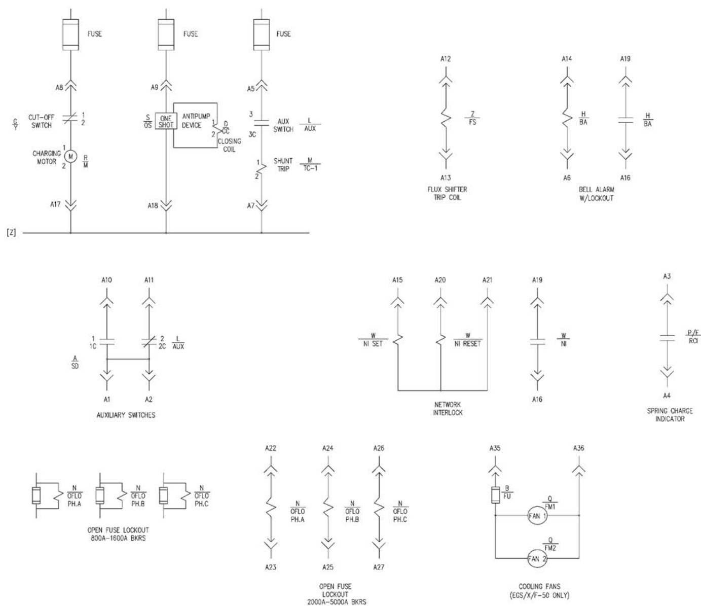
Figure 5.3 Wiring Diagram
