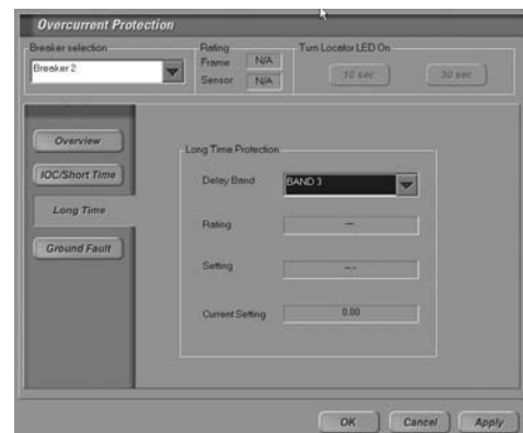
Figure 13.11 Long-time Overcurrent Protection Setting Display
